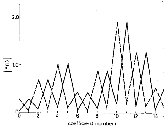
Fig. 10 As Fig. 5, but using the WHT
