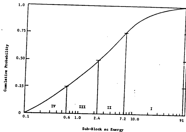
Figure 4. Probability distribution of sub-block ac energy.
