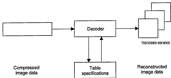
Figure 2 - Decoder
