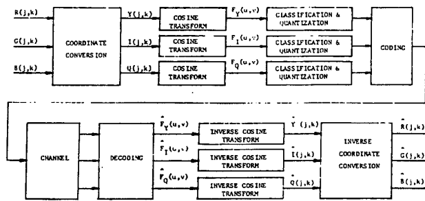
Figure 7. Cosine transform color image coding system.
