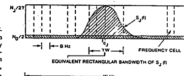
Fig. 2. AWGN plus realistic partial-band jamming power spectral density with Gaussian-shape.
