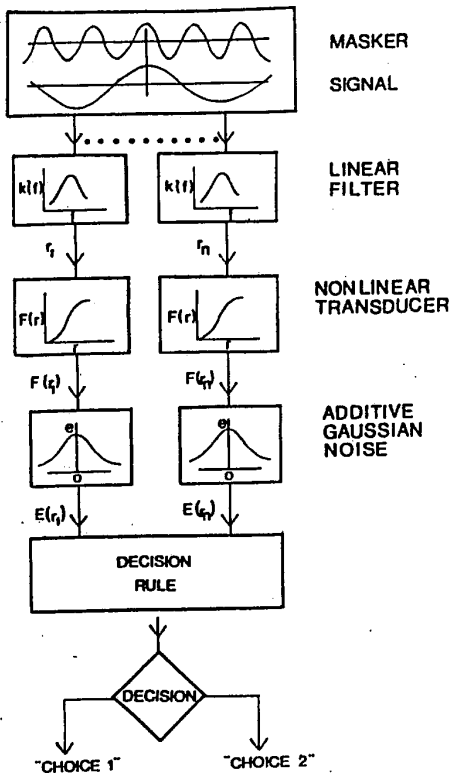
FIG. 7. Schematic representation of the masking model.
