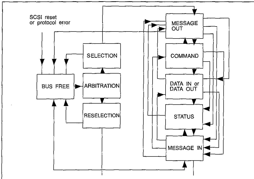
Figure 10.12 Complete SCSI phase diagram.
