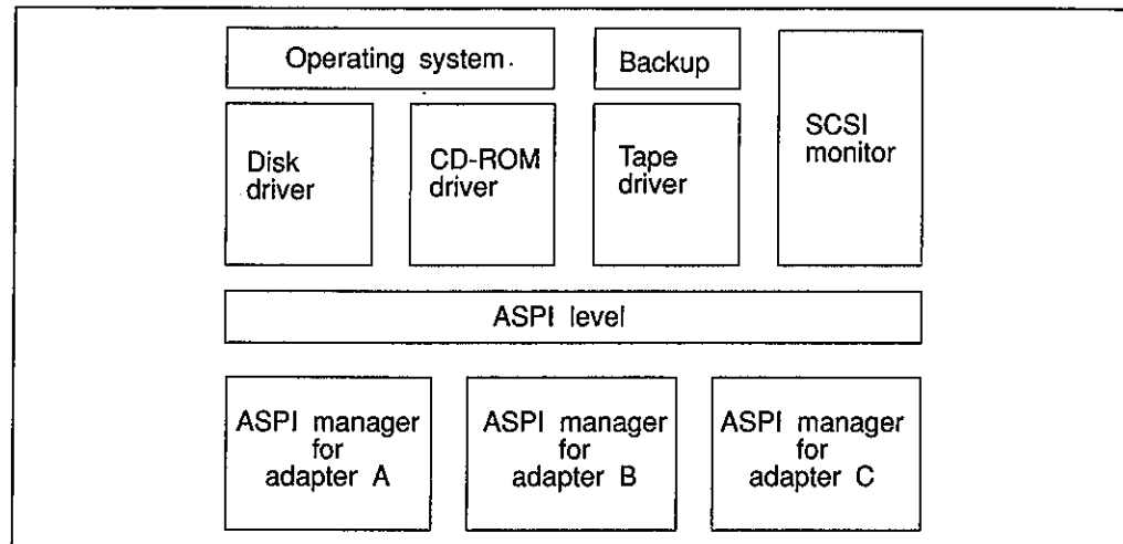
Figure 23.1 ASPI functional overview.
