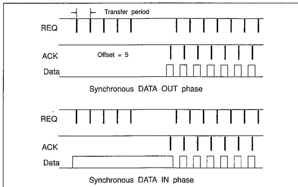
Figure 10.22 Synchronous data phases.
