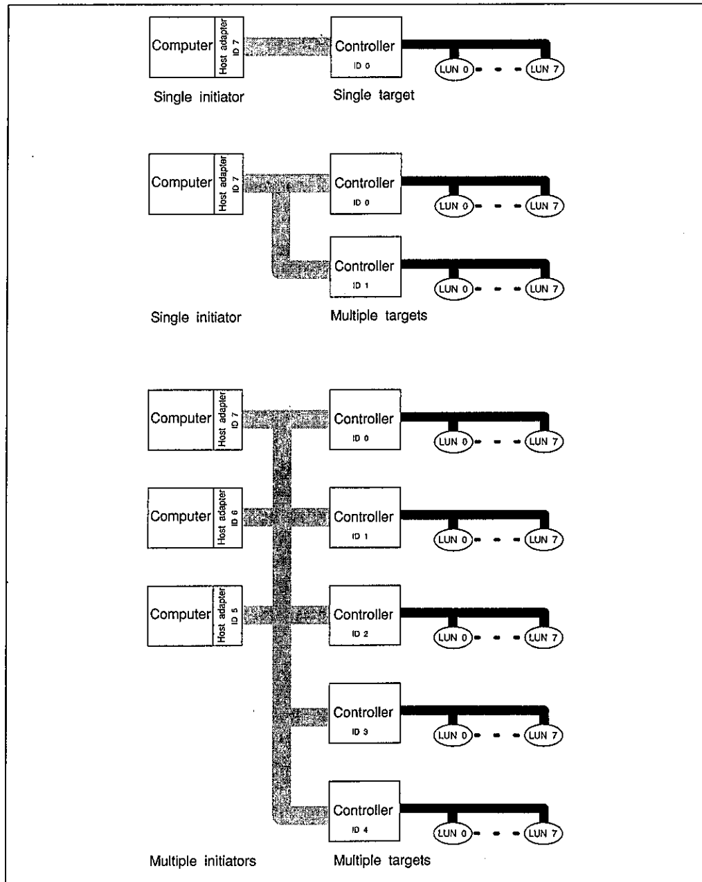
Figure 10.3 Basic SCSI configurations.
