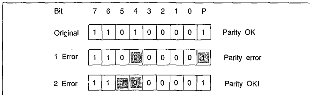
Figure 10.7 Shortcomings of SCSI parity.
