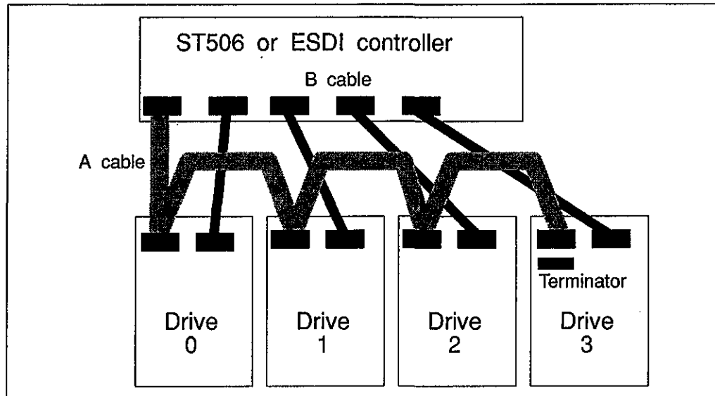
Figure 2.8 ST506 configuration.
