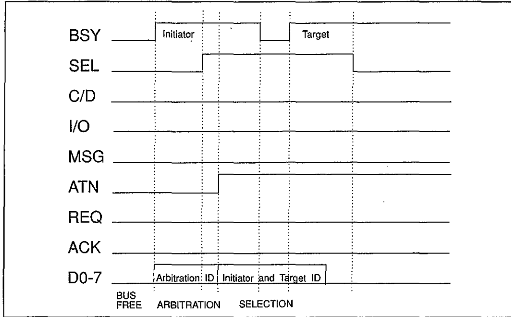
Figure 10.14 ARBITRATION and SELECTION.
