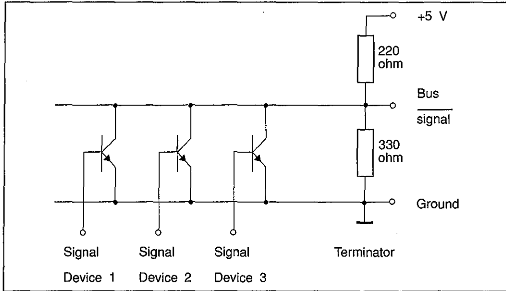
Figure 10.4 Wired-or bus signals.
