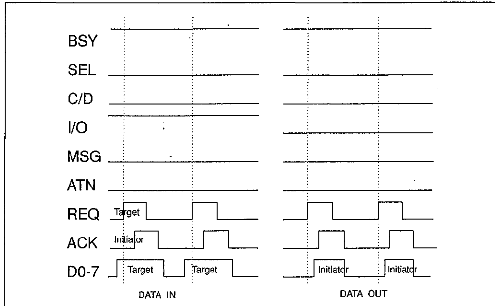
Figure 10.19 DATA IN and DATA OUT.
