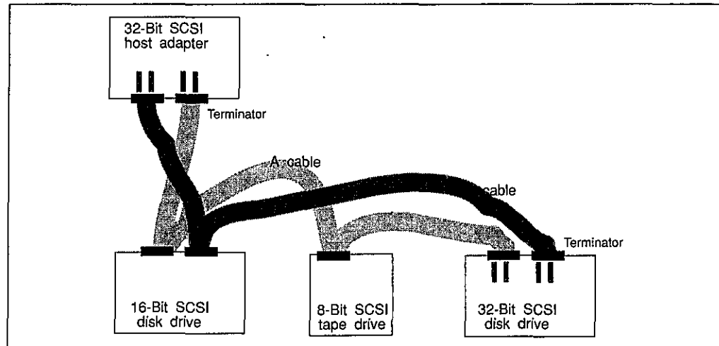
Figure 10.6 Mixed configuration with Wide SCSI.
