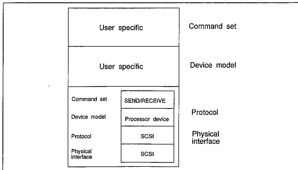
Figure 17.1 User defined protocol.
