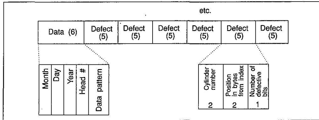
Figure 2.13 ESDI defect list.
