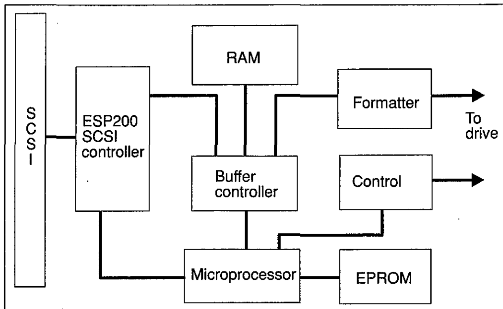
Figure 25.1 Typical target application using ESP200.
