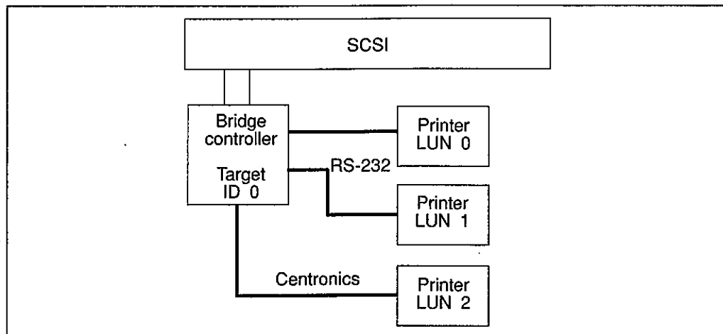
Figure 9.2 Bridge controller with logical units.
