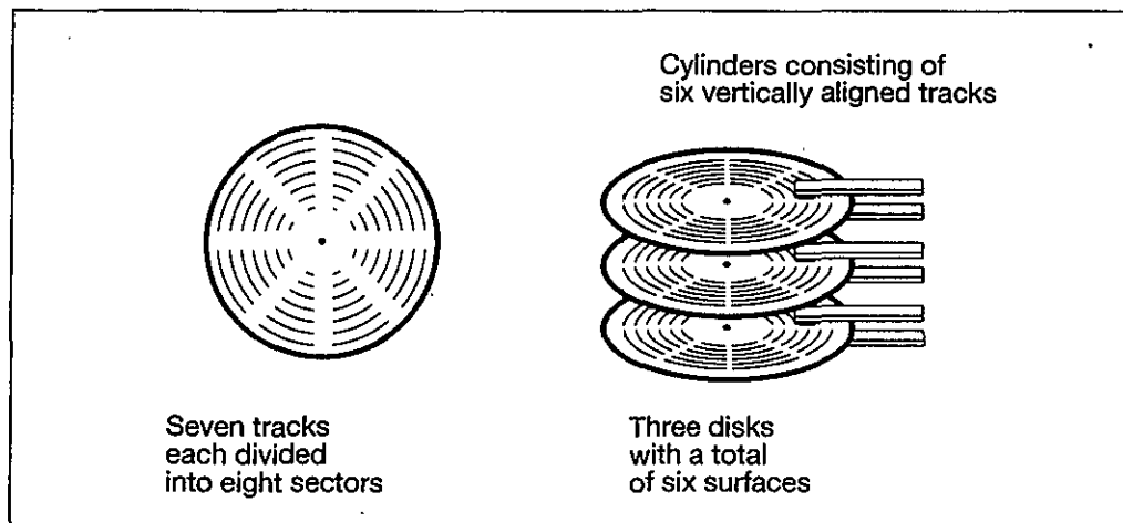
Figure 2.4 Structure of disk medium.
