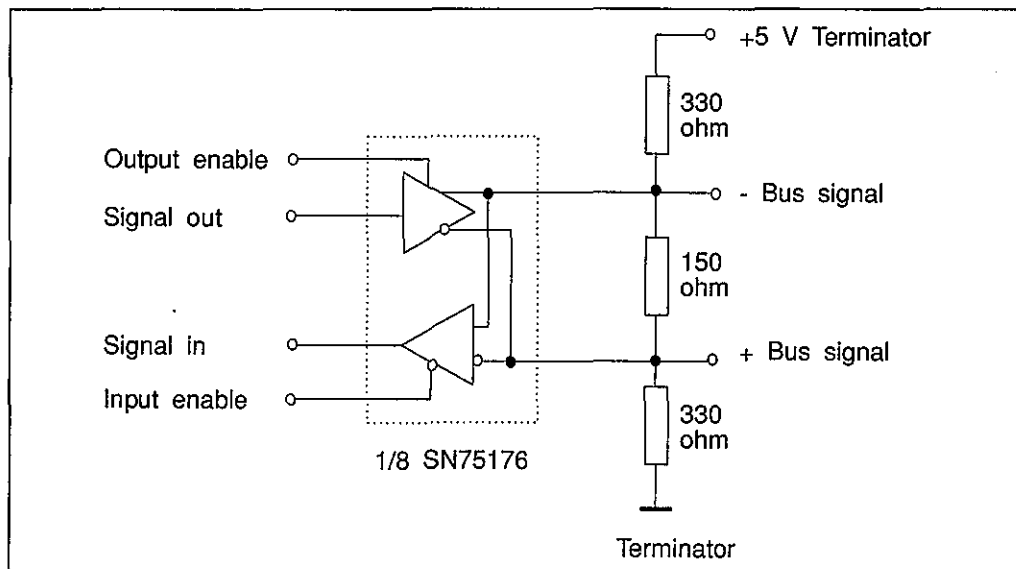
Figure 10.10 Differential SCSI drivers.
