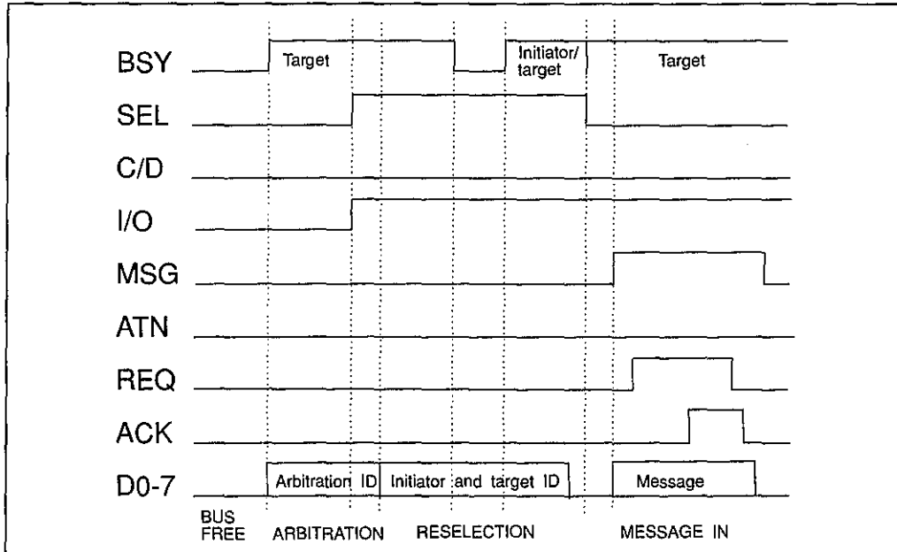
Figure 10.16 RESELECTION and MESSAGE IN.
