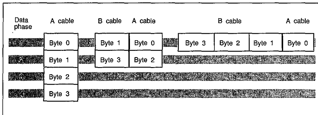
Figure 10.5 Byte ordering for Wide SCSI.
