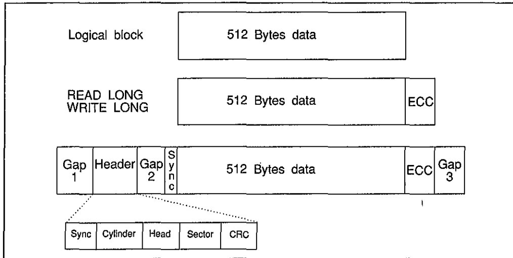
Figure 13.3 Physical layout of a logical block.
