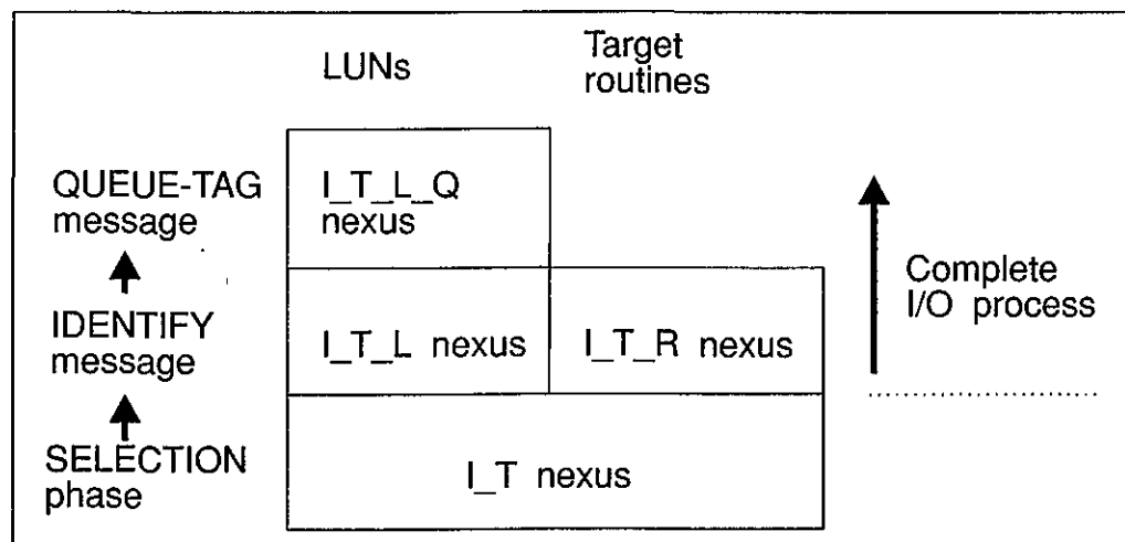
Figure 11.2 Structure of a nexus.
