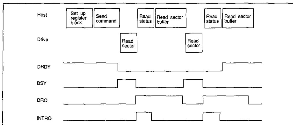
Figure 6.1 Timing of a class 1 command.
