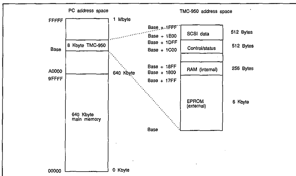
Figure 25.3 Address space of TMC-950.
