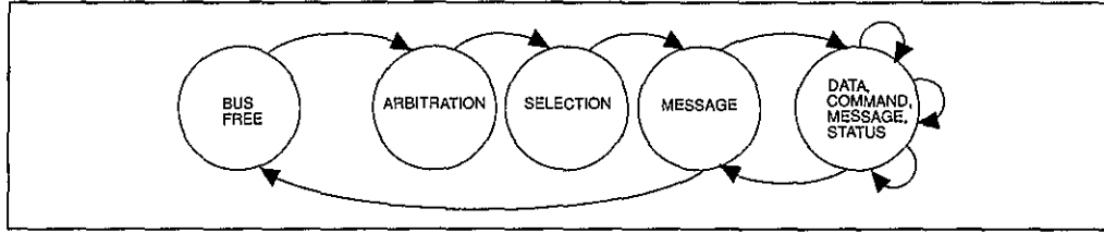
Figure 10.11 Simplified SCSI phase diagram.
