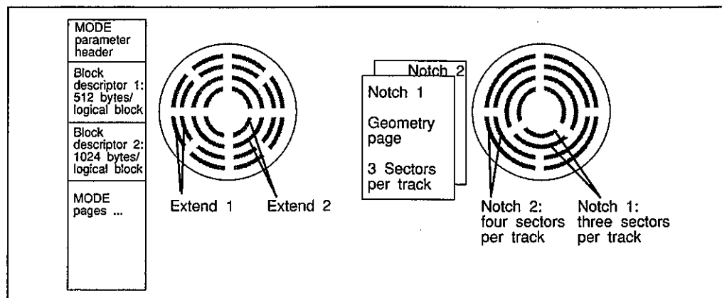
Figure 13.2 SCSI extends and notches.
