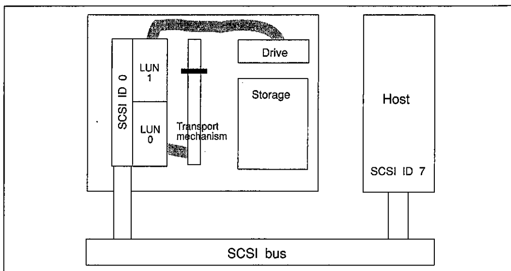
Figure 21.2 SCSI medium-changer configuration.
