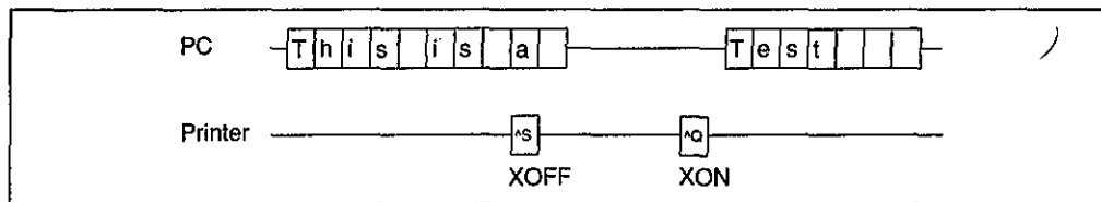
Figure 2.2 XON/XOFF protocol.
