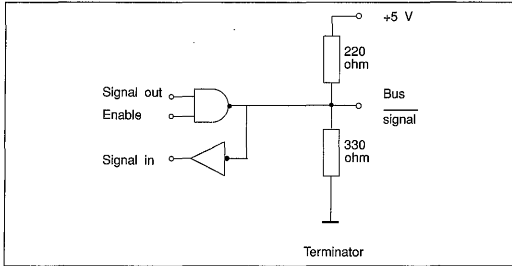
Figure 10.8 Typical single-ended SCSI.
