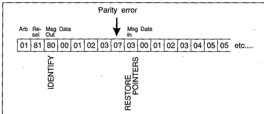
Figure 11.1 Parity error.
