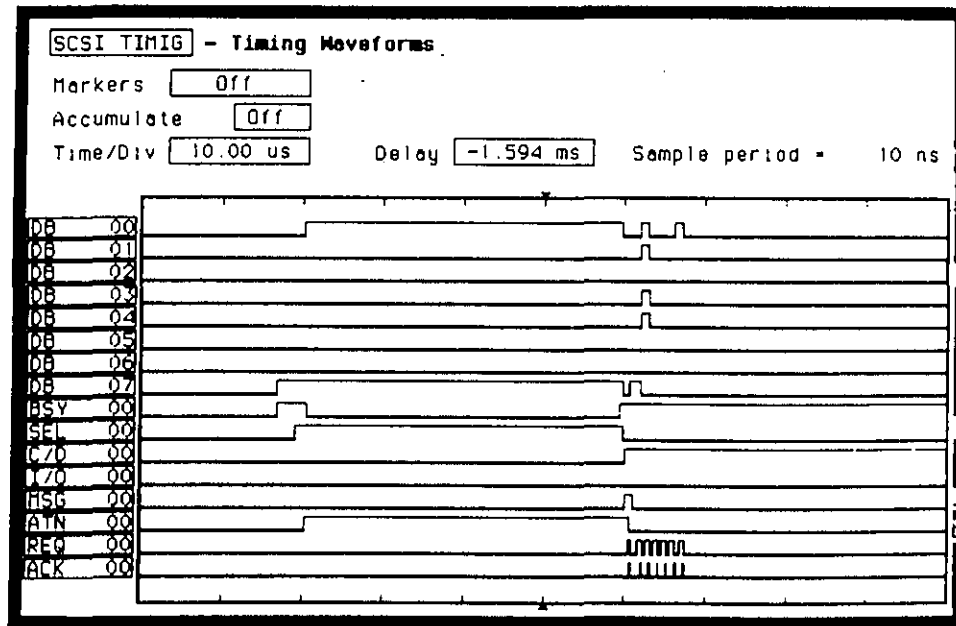
Figure 24.1 SCSI timing diagram.
