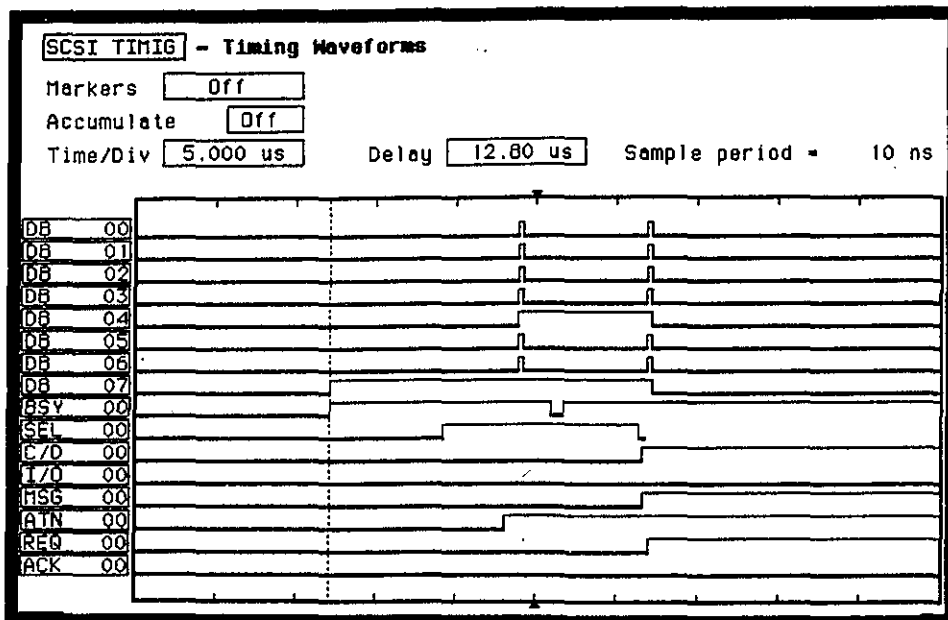
Figure 10.15 ARBITRATION and SELECTION as seen on a logic analyzer.
