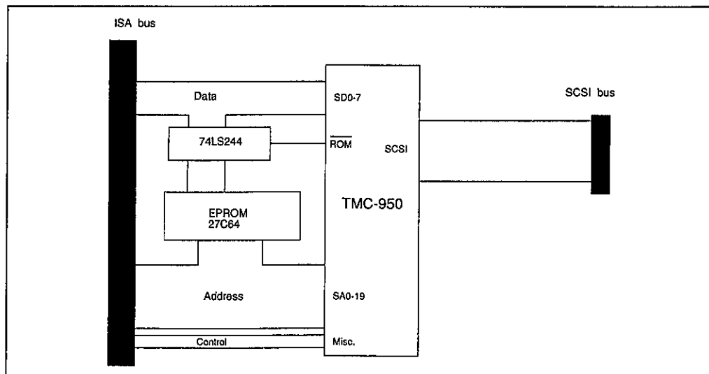
Figure 25.2 Three-chip PC host adaptor using TMC-950.
