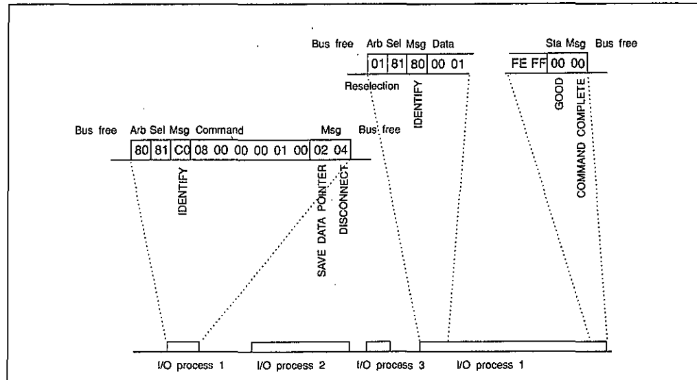
Figure 11.3 Freeing the bus and reselection.
