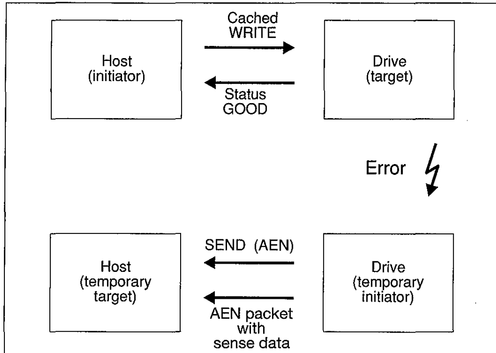
Figure 11.5 Asynchronous event notification.
