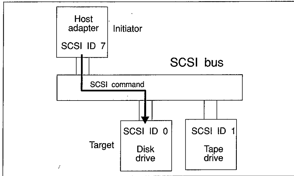
Figure 9.1 A simple SCSI configuration.
