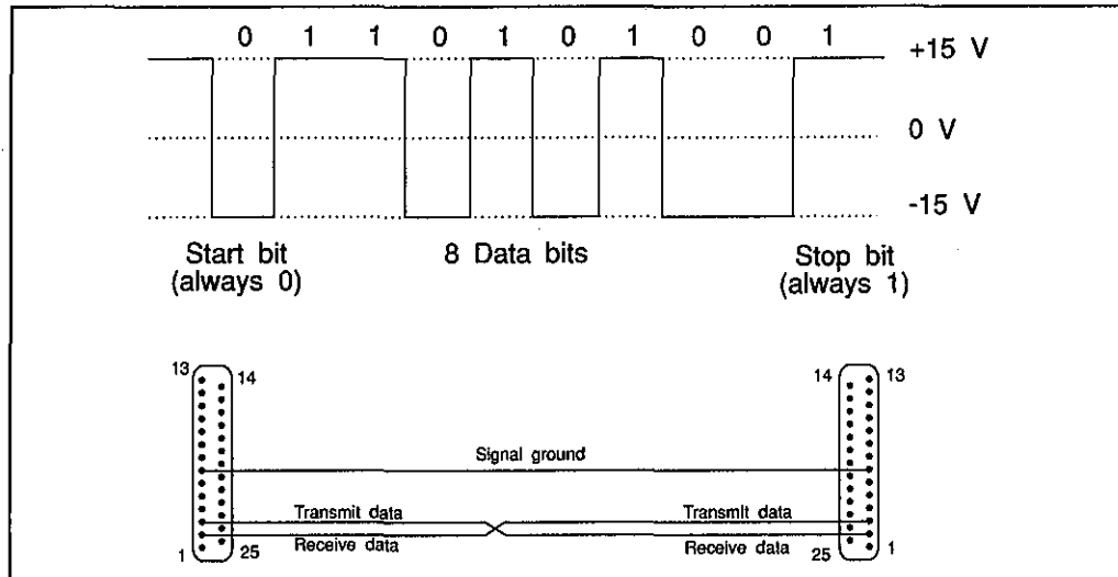
Figure 2.1 Physical interface: mini-RS-232.
