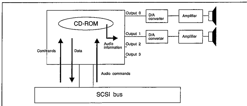
Figure 20.1 Model of a CD-ROM drive.
