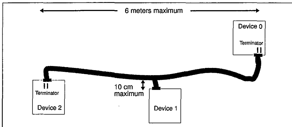
Figure 9.3 SCSI cable.
