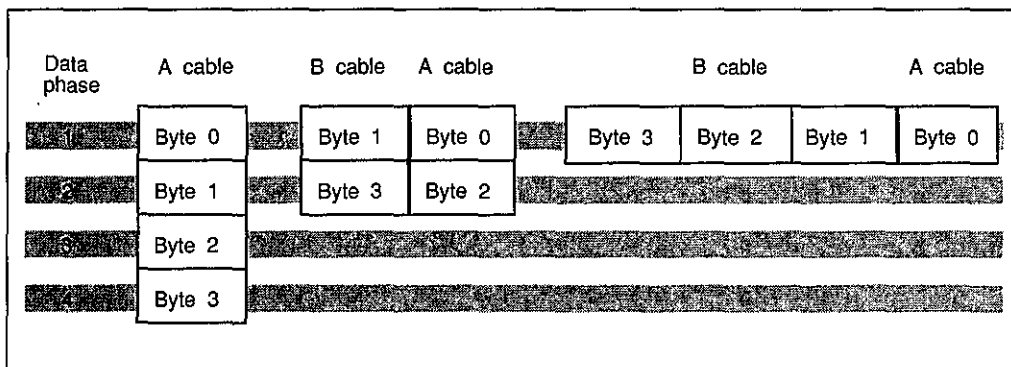
Figure 10.5 Byte ordering for Wide SCSI.
