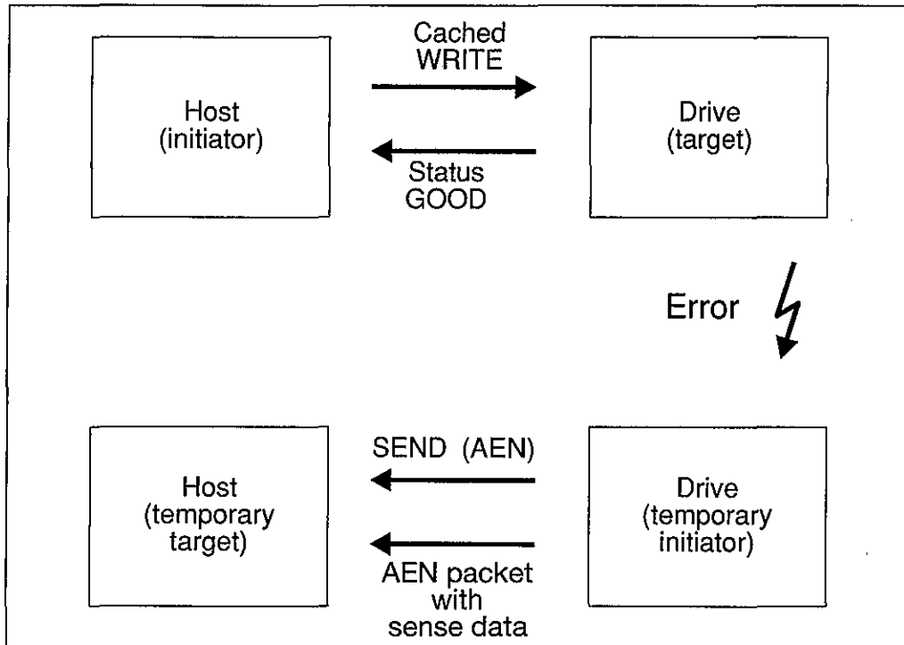
Figure 11.5 Asynchronous event notification.
