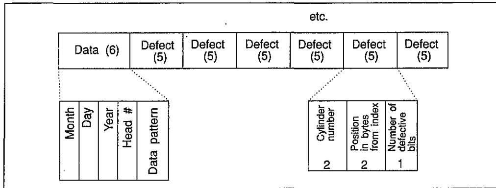
Figure 2.13 ESDI defect list.
