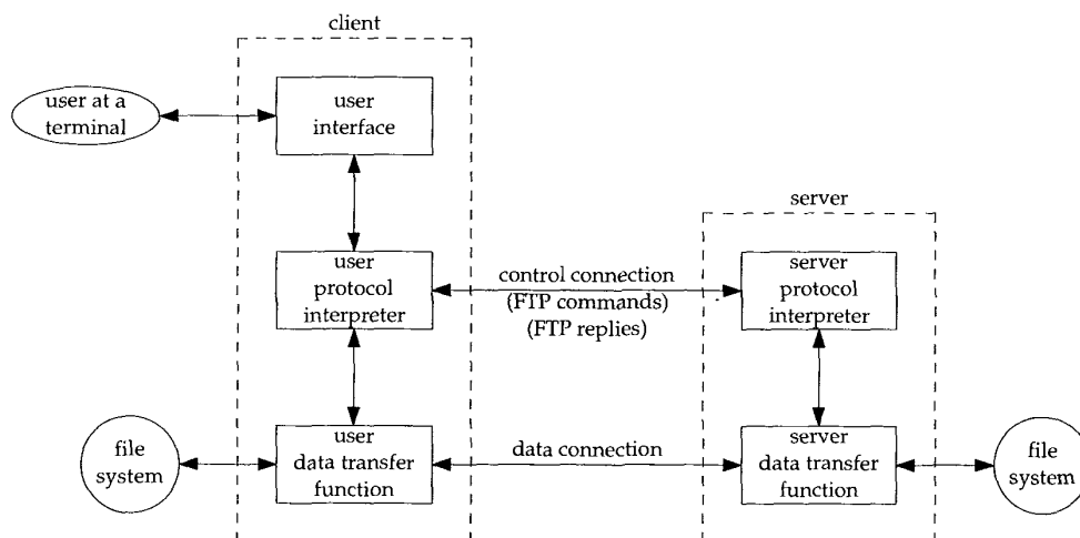
Figure 27.1 Processes involved in file transfer.
