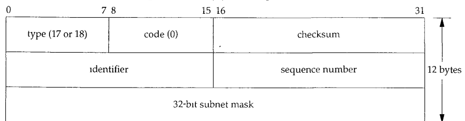
Figure 6.4 ICMP address mask request and reply messages.
