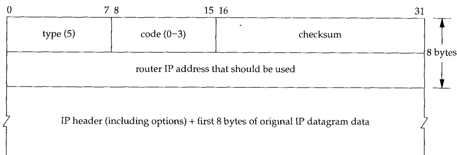
Figure 9.4 ICMP redirect message.
