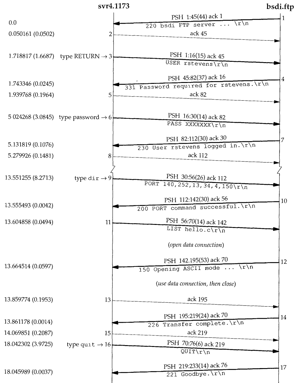
Figure 27.6 Control connection for FTP example.
