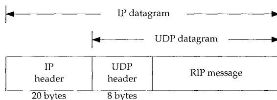
Figure 10.2 RIP message encapsulated within a UDP datagram.
