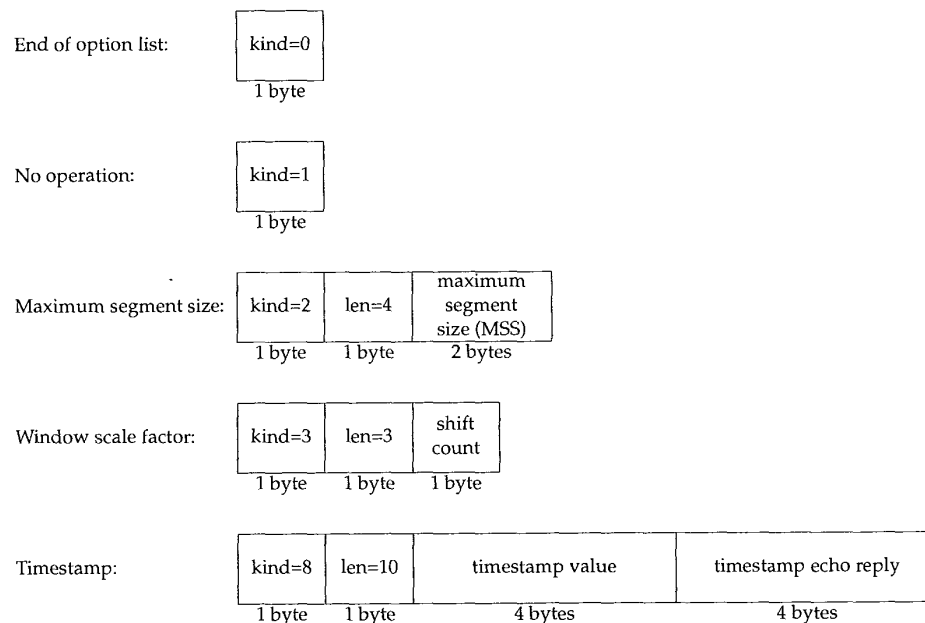
Figure 18.20 TCP options.
