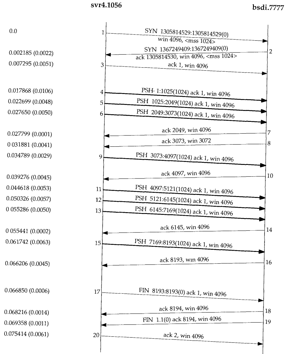
Figure 20.1 Transfer of 8192 bytes from svr4 to bsd1.
