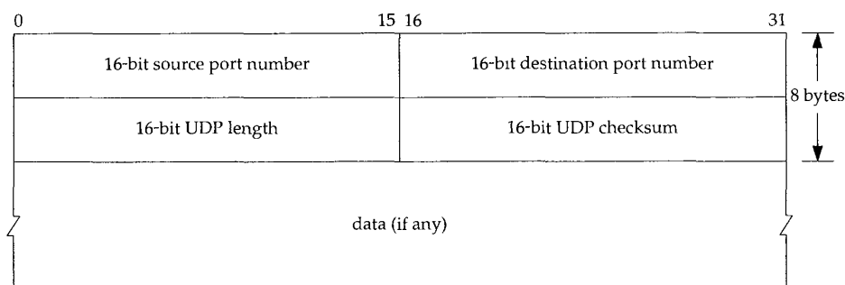
Figure 11.2 UDP header.
