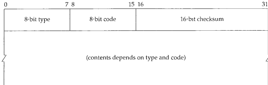
Figure 6.2 ICMP message.
