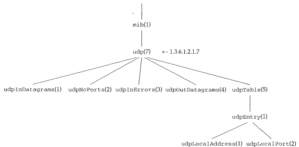
Figure 25.7 Tree structure of UDP group.
