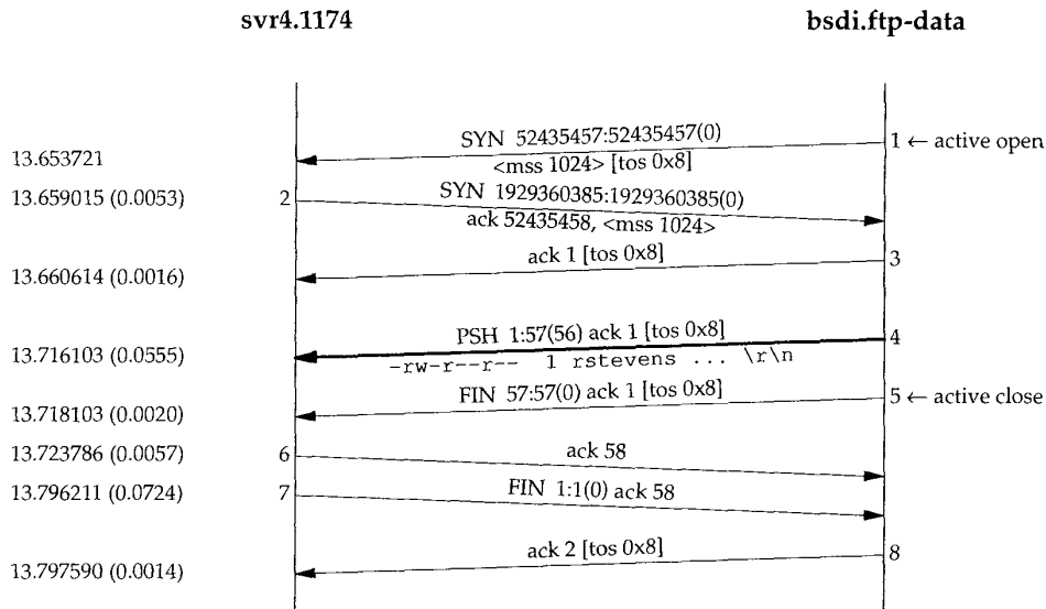
Figure 27.7 Data connection for FTP example.
