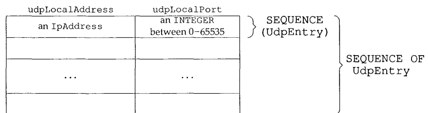
Figure 25.5 UDP listener table ( udpTable ) as a two-dimensional array in SNMP.
