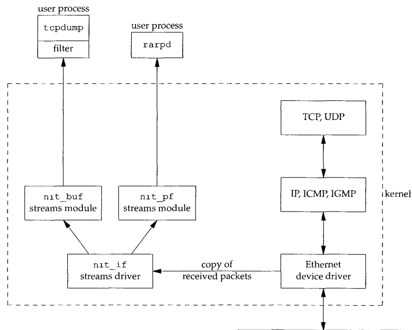
Figure A.2 SunOS Network Interface Tap.
