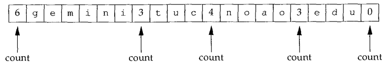
Figure 14.6 Representation of the domain name gemini.tuc.noao.edu .
