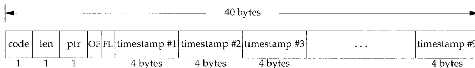
Figure 7.7 General format of timestamp option in IP header.
