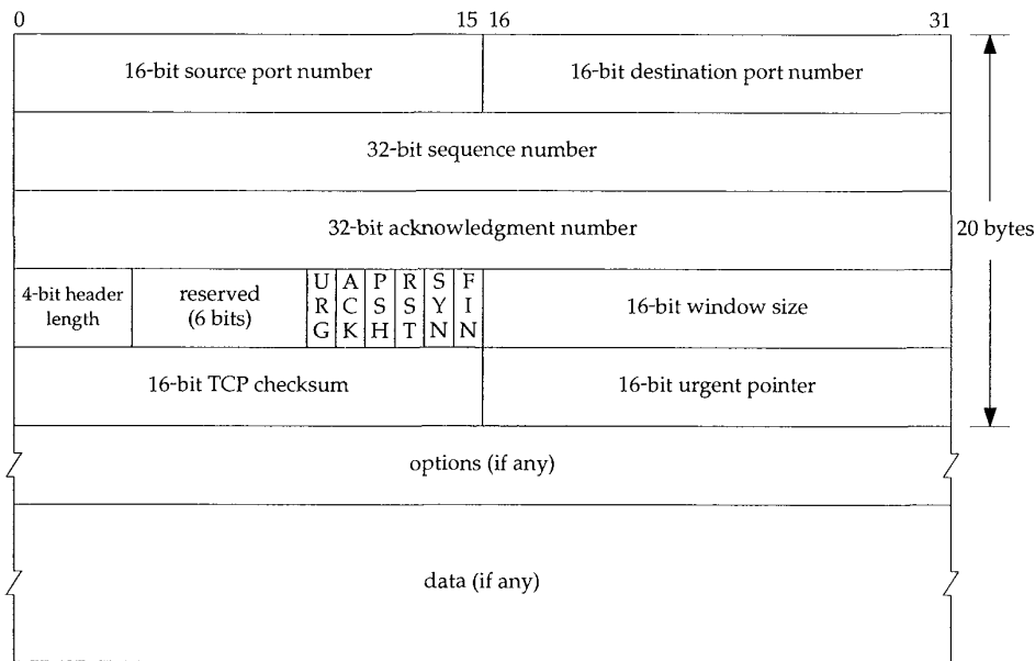
Figure 17.2 TCP header.
