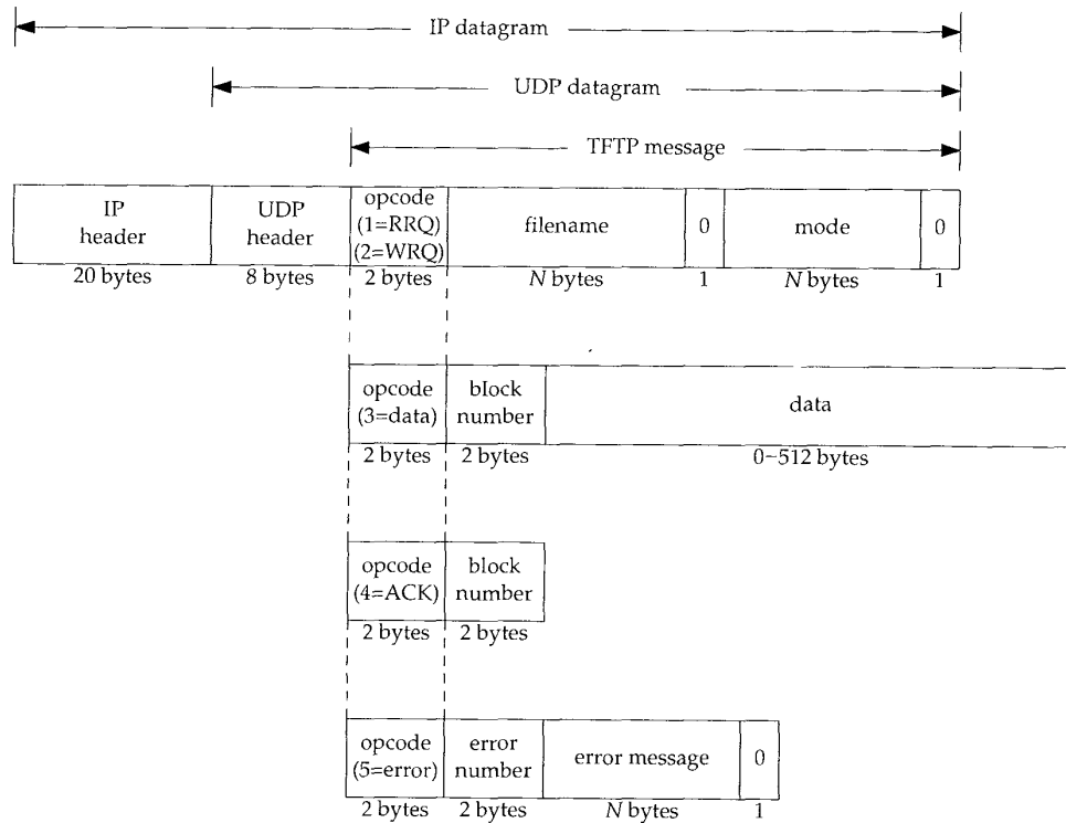
Figure 15.1 Format of the five TFTP messages.
