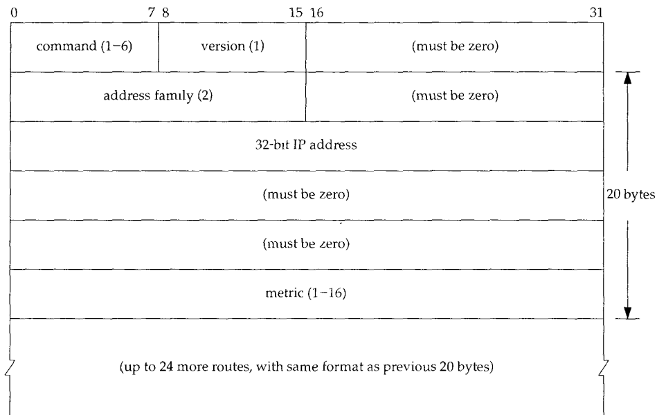
Figure 10.3 Format of a RIP message.
