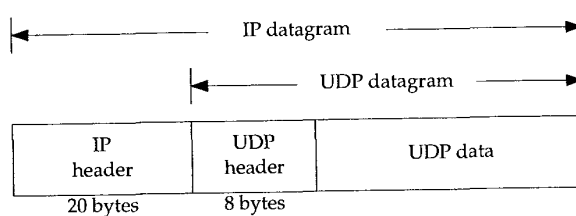
Figure 11.1 UDP encapsulation.
