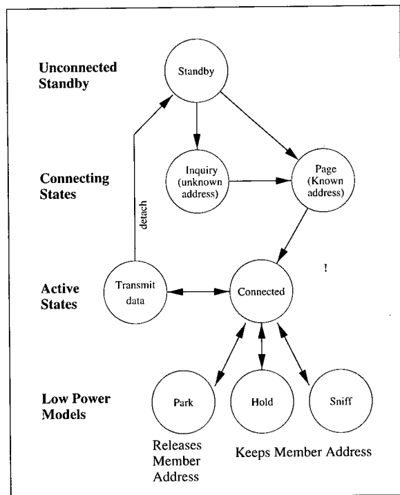
Figure 3: Connection State Machine
