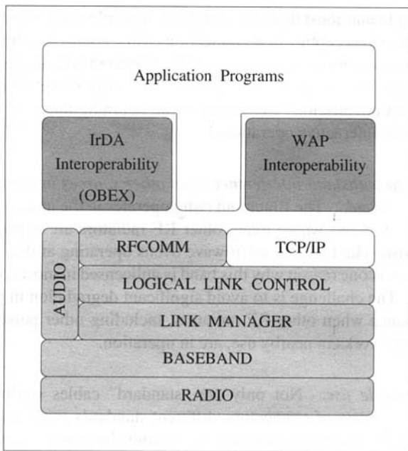
Figure 1: Application Framework
