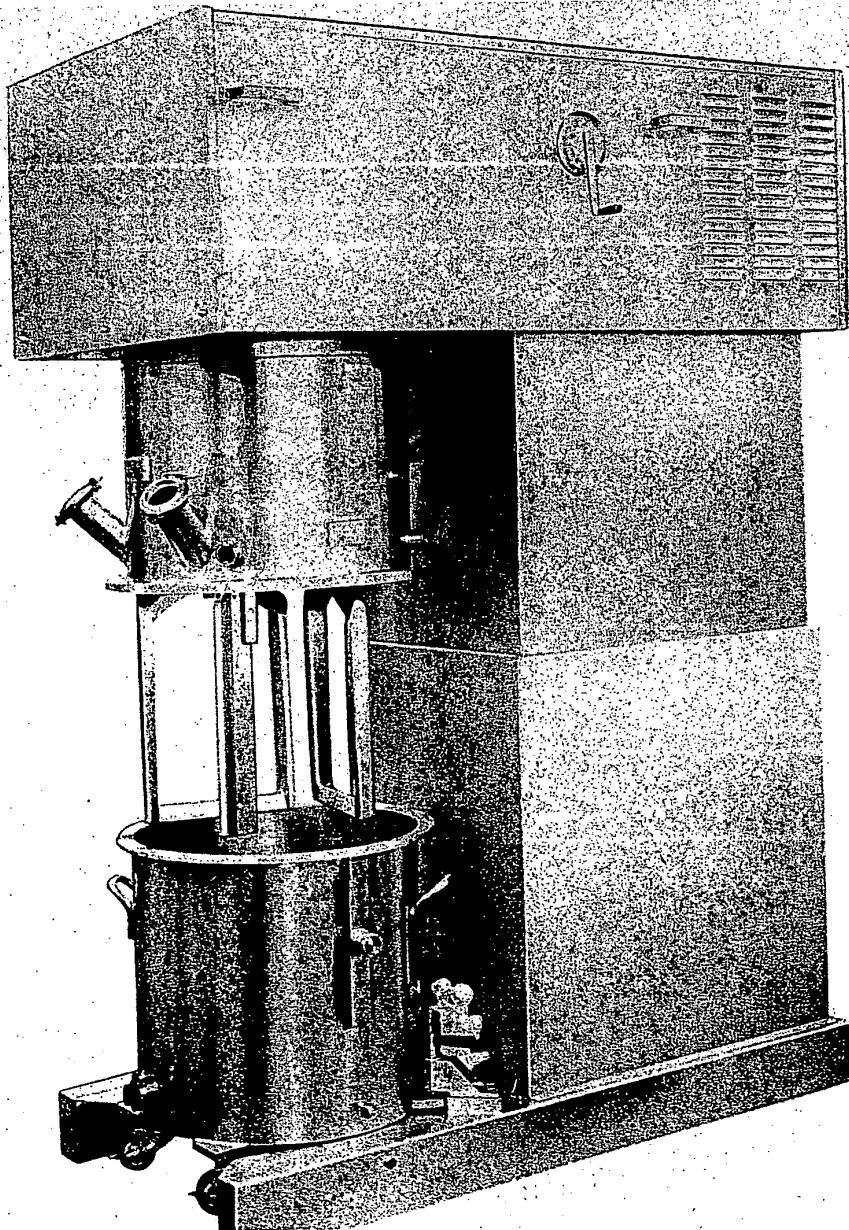
Figure 5 Ross HDM 40 sanitary double planetary mixer. (Courtesy of Charles Ross & Son Co., Happauge, New York.)
