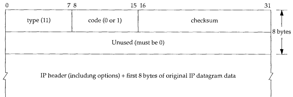
Figure 8.2 ICMP time exceeded message.
