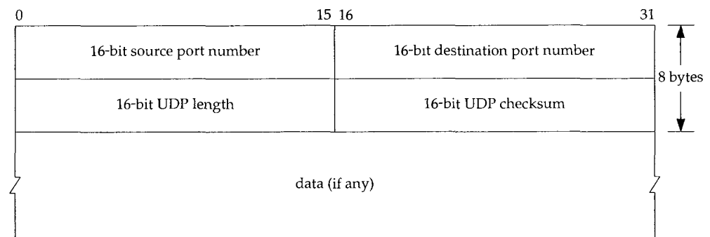
Figure 11.2 UDP header.
