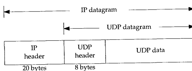
Figure 11.1 UDP encapsulation.
