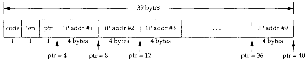
Figure 7.3 General format of record route option in IP header.
