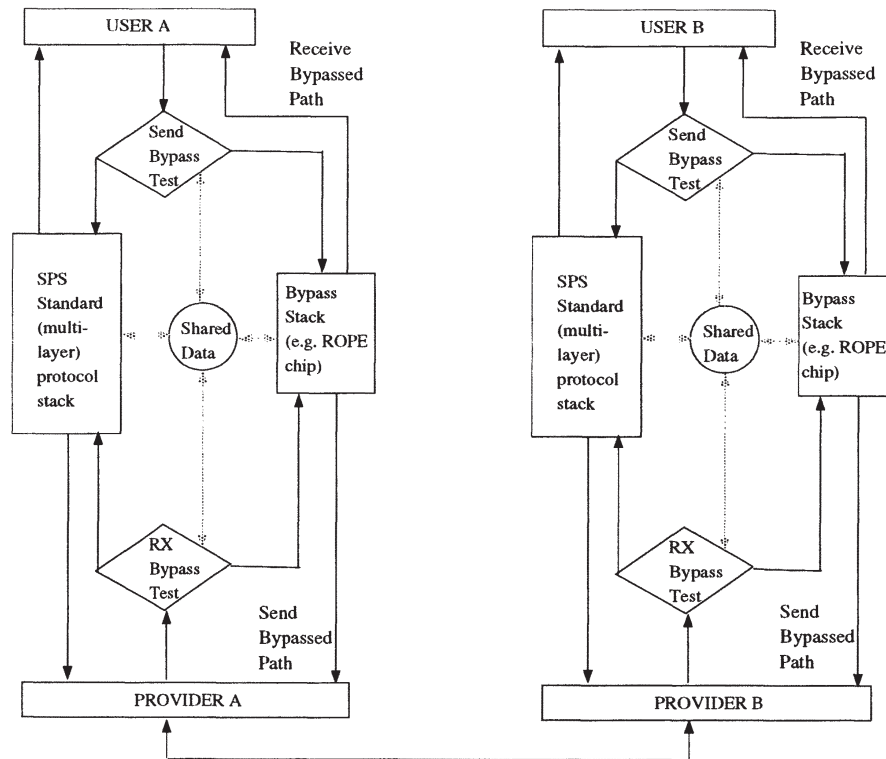
Figure 1 Bypass Architecture
