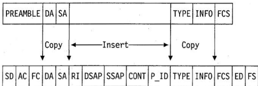
Figure 5-15. 8229 TCP/IP Support. Conversion process.
