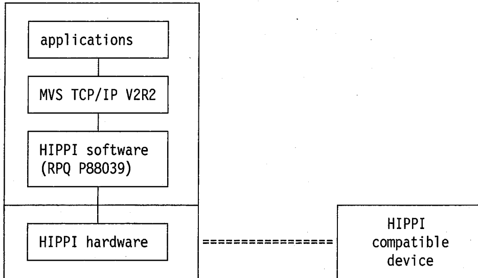
Figure 5-5. IBM HIPPI and MVS TCP/IP
