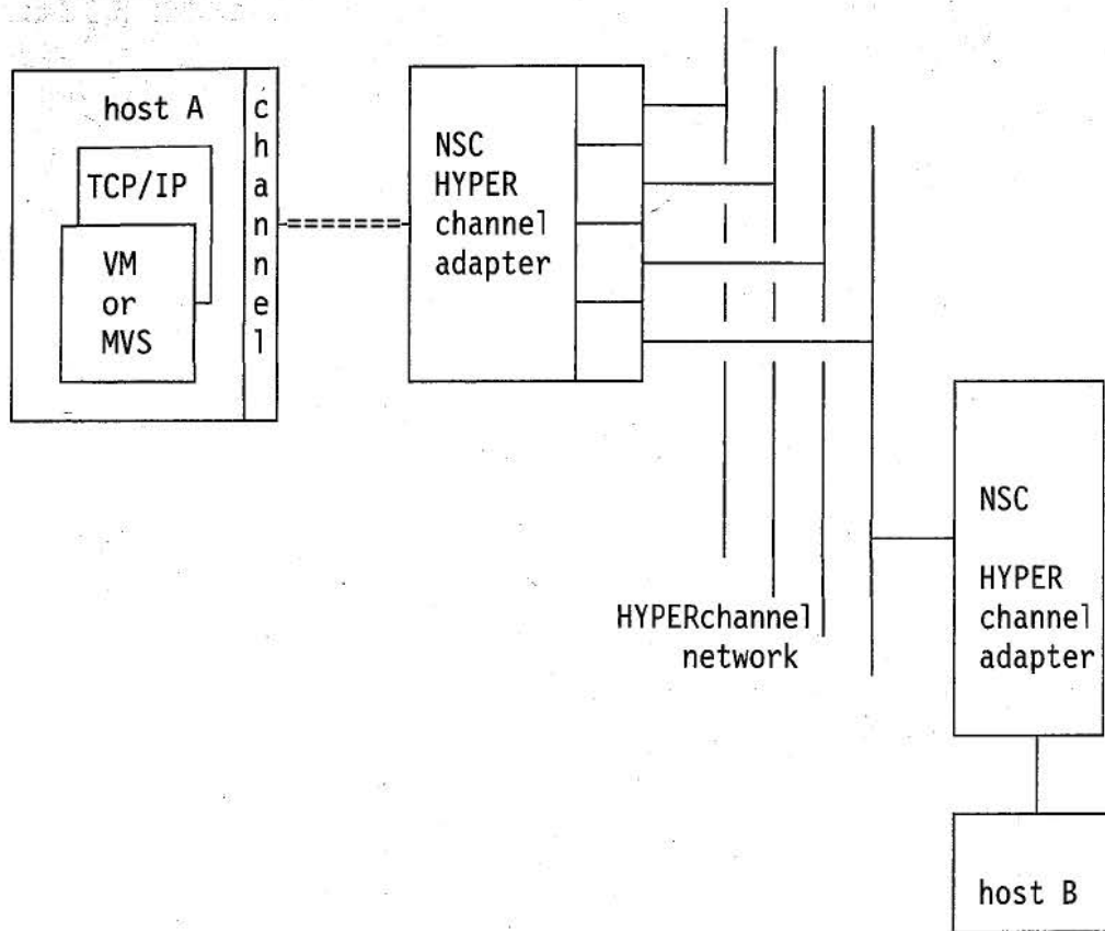
Figure 5-4. HYPERchannel Network
