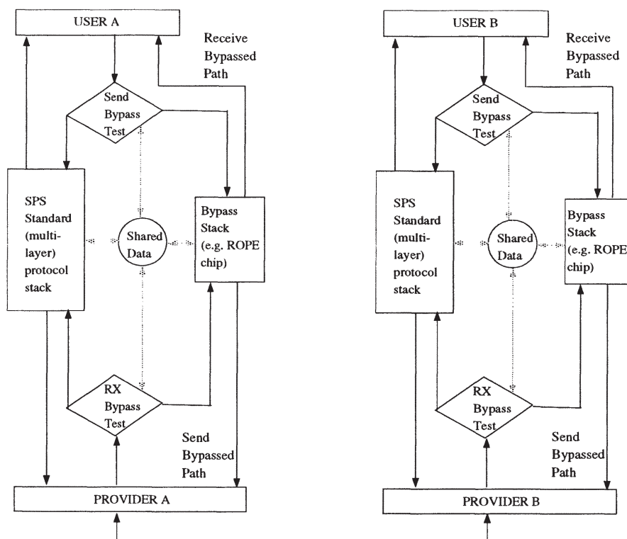
Figure 1 Bypass Architecture
