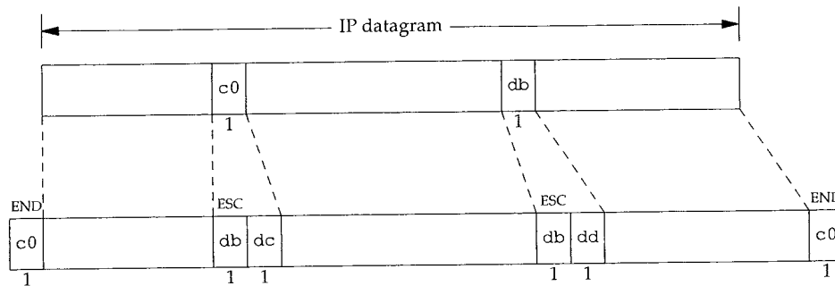
Figure 2.2 SLIP encapsulation.
