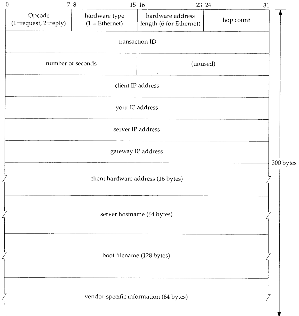
Figure 16.2 Format of BOOTP request and reply.
