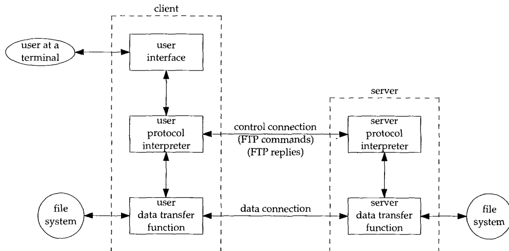
Figure 27.1 Processes involved in file transfer.
