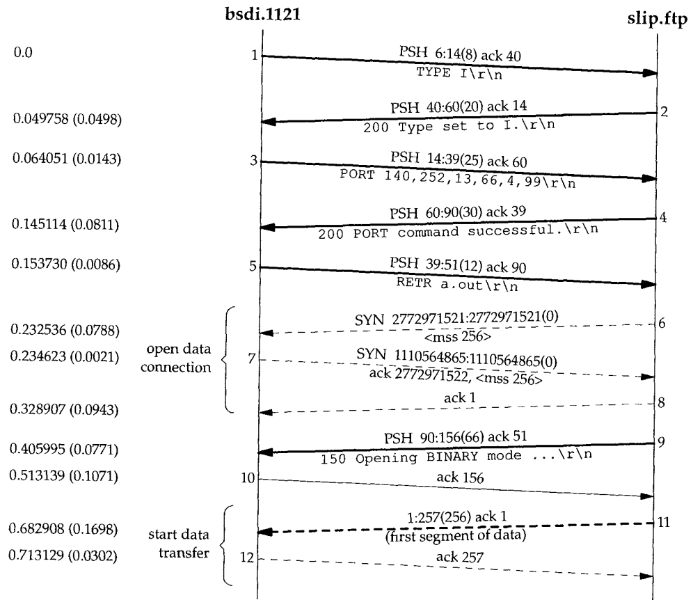
Figure 27.9 Aborting a file transfer (first half).
