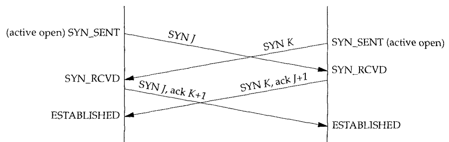
Figure 18.17 Segments exchanged during simultaneous open.
