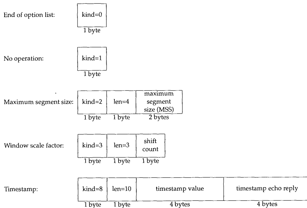
Figure 18.20 TCP options.
