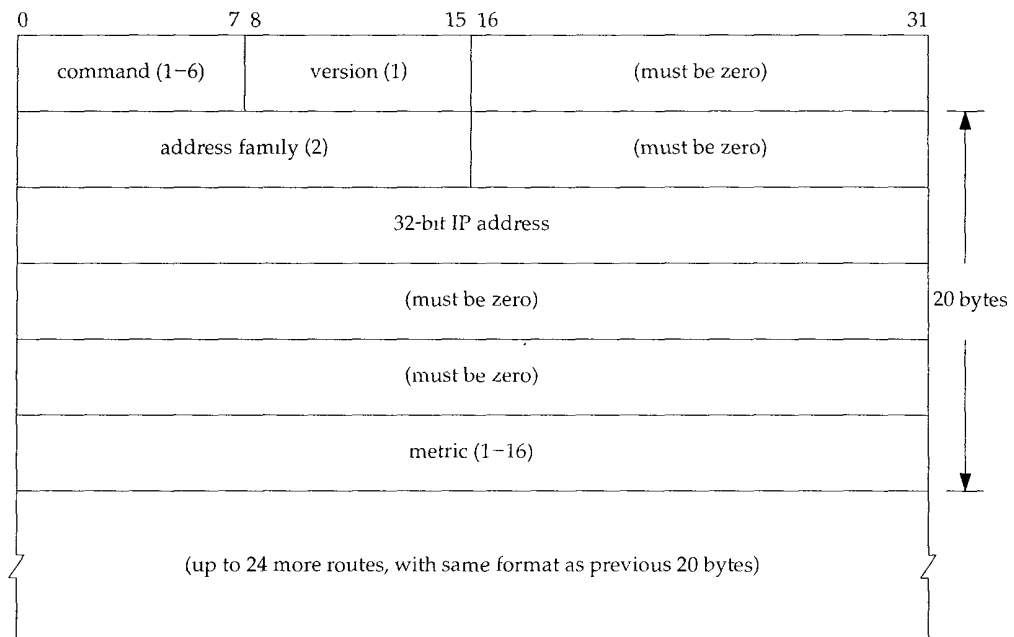
Figure 10.3 Format of a RIP message.
