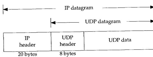
Figure 11.1 UDP encapsulation.
