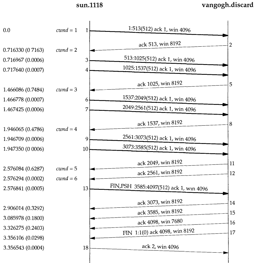
Figure 20.8 Example of slow start.
