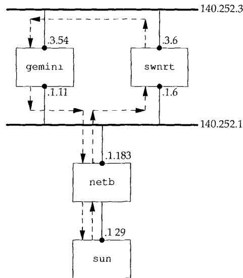
Figure 25.29 Topology of systems being used for example.
