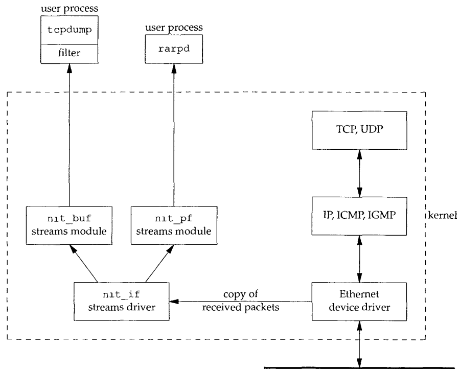
Figure A.2 SunOS Network Interface Tap.
