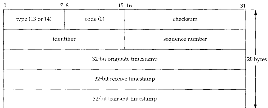
Figure 6.6 ICMP timestamp request and reply messages.
