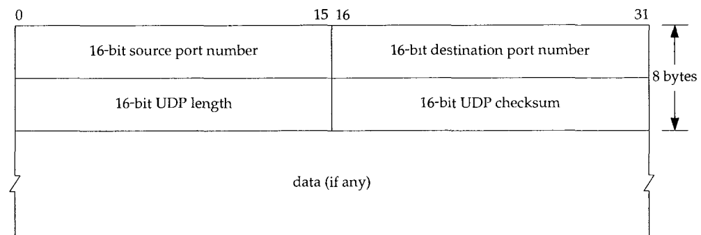
Figure 11.2 UDP header.
