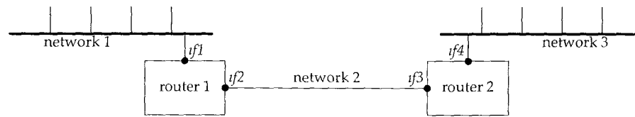
Figure 8.3 Identification of interfaces printed by traceroute.
