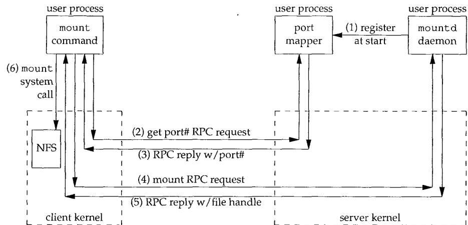
Figure 29.5 Mount protocol used by Unix mount command.
