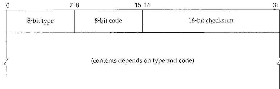
Figure 6.2 ICMP message.
