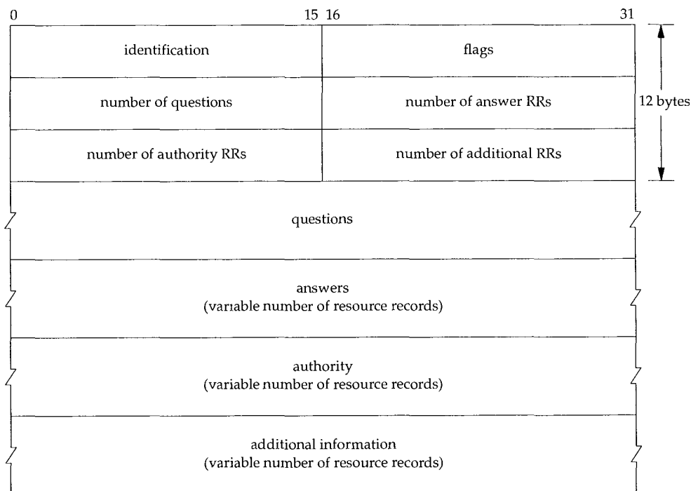
Figure 14.3 General format of DNS queries and responses.
