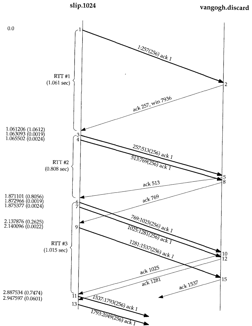
Figure 21.2 Packet exchange and RTT measurement.
