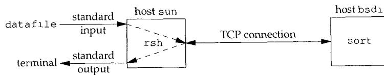
Figure 18.11 The command: rsh bsd1 sort < datafile .
