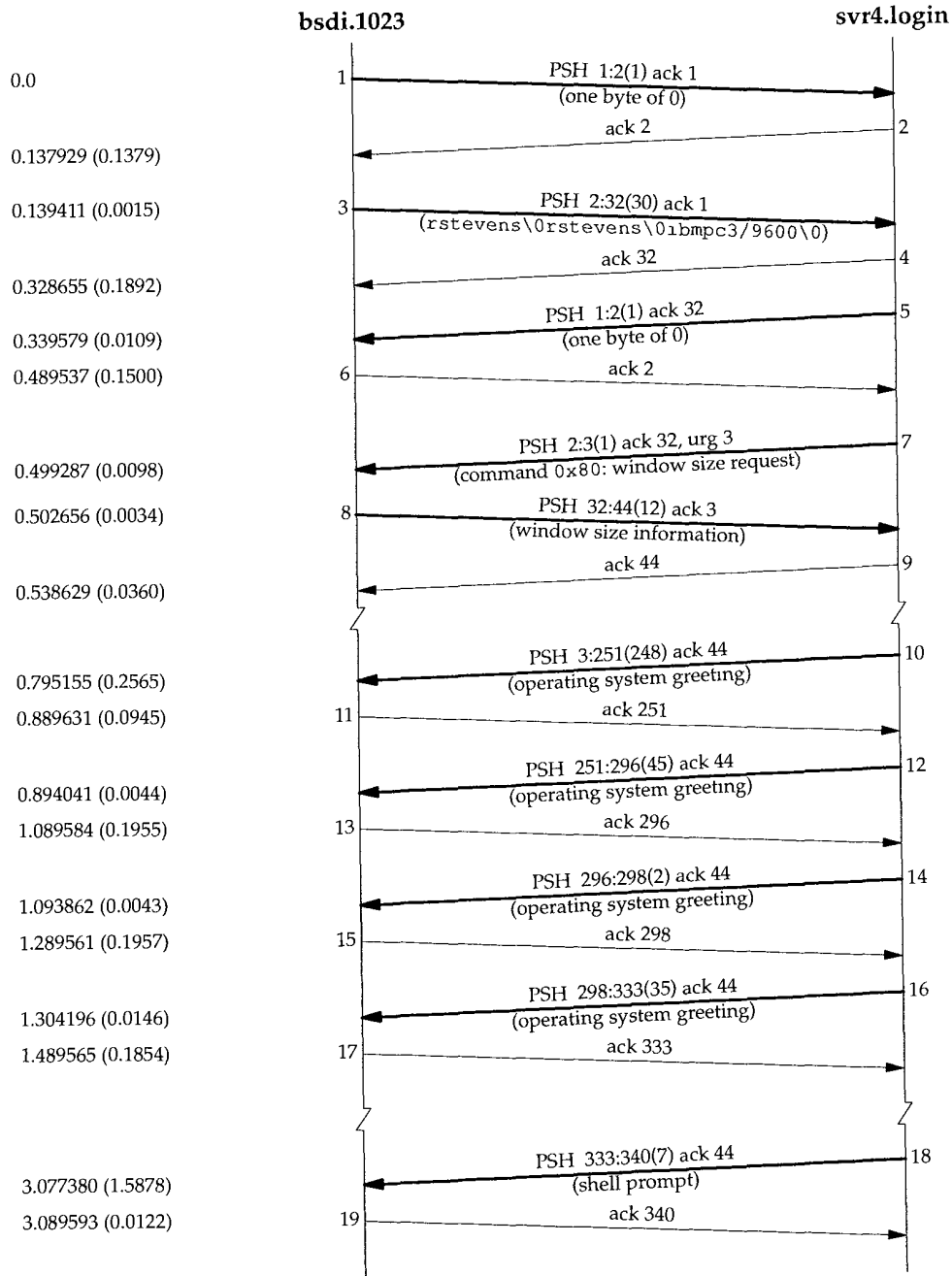
Figure 26.5 Time line for an Rlogin connection.
