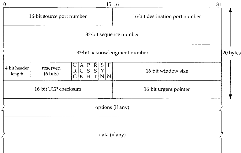
Figure 17.2 TCP header.
