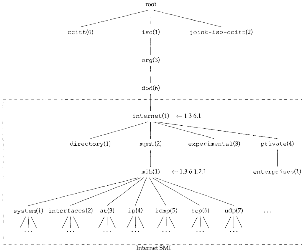
Figure 25.6 Object identifiers in the Management Information Base.
