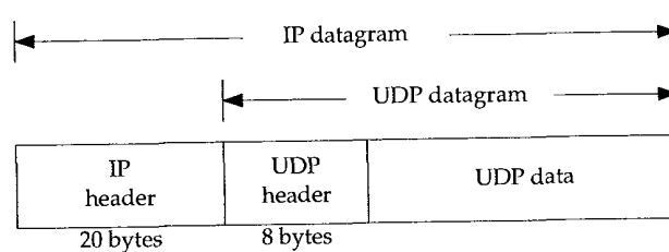
Figure 11.1 UDP encapsulation.
