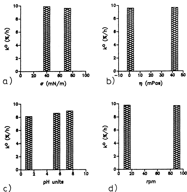
Fig. 2. Comparison of the in vitro drug release of IS-5-N depending on different dissolution models. k^0 , zero-order release constant. (a) Rotating bottle, influence of surface tension. (b) Rotating bottle, influence of viscosity. (c) Rotating bottle, influence of pH variation. (d) Paddle apparatus, influence of hydrodynamics.
