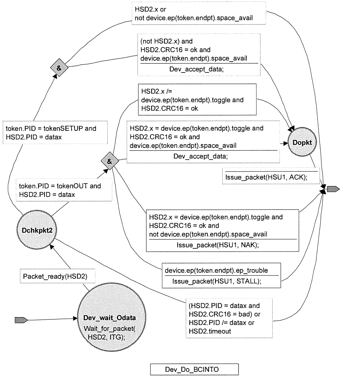
Figure 8-32. Bulk/Control/Interrupt OUT Transaction Device State Machine
