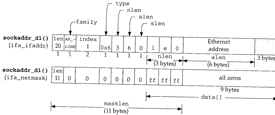
Figure 3.38 The initialized Ethernet sockaddr_dl structures (sdl_ prefix omitted).
