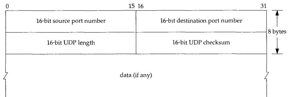
Figure 11.2 UDP header.
