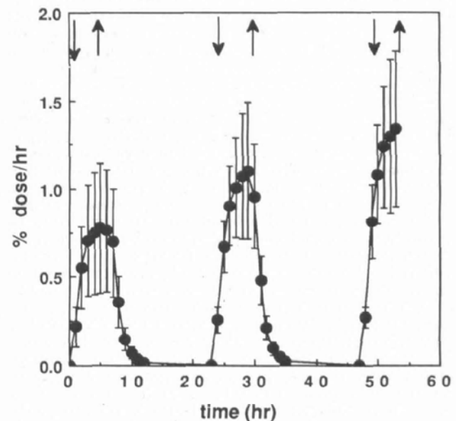
Figure 5. Tritiated water flux (mean \pm SD, n = 4 ) across hairless mouse skin after applications from t = 0-5 h, t = 24-29 h, and t = 48-53 h. Before each administration of water, the skin was pretreated with acetone at a dose of 15 \mu\text{l}/\text{cm}^2 .
