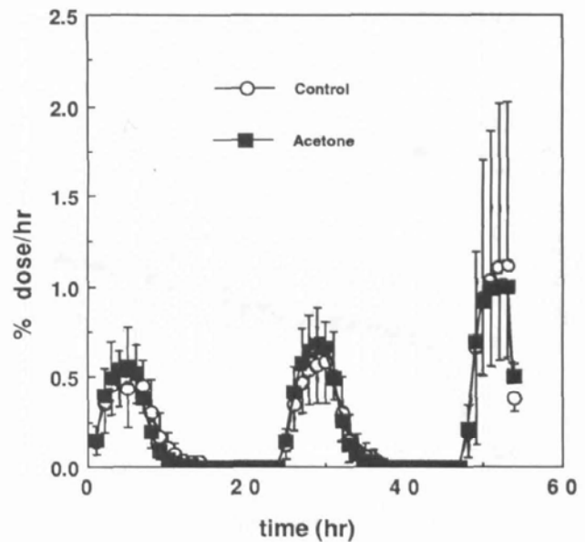
Figure 4. Effect of acetone pretreatment ( 15 \mu\text{l}/\text{cm}^2 ) on tritiated water flux (mean \pm SD, n \geq 12 ) across hairless mouse skin after applications from t = 0-5 h, t = 24-29 h, and t = 48-53 h (experiment IV).
