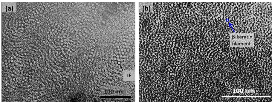
Fig. 3. Transmission electron micrographs of typical keratinous materials with clear filament-matrix structure: (a) cross section of a human hair ( \alpha -keratin), stained with osmium tetroxide, showing 7 nm diameter intermediate filaments embedded in a darker matrix; (b) cross section of a seagull feather rachis ( \beta -keratin), stained with potassium permanganate, showing the 3.5 nm diameter \beta -keratin filaments differentiated by the densely stained matrix [16].
