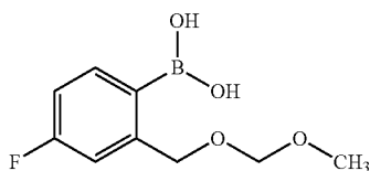
[[4-Fluoro-2-methoxymethoxymethyl]phenyl]boronic acid
