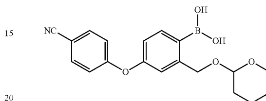
[[4-[4-cyanophenoxy]-2-[(tetrahydro-2H-pyran-2-yl)oxy]methyl]phenyl]boronic acid
