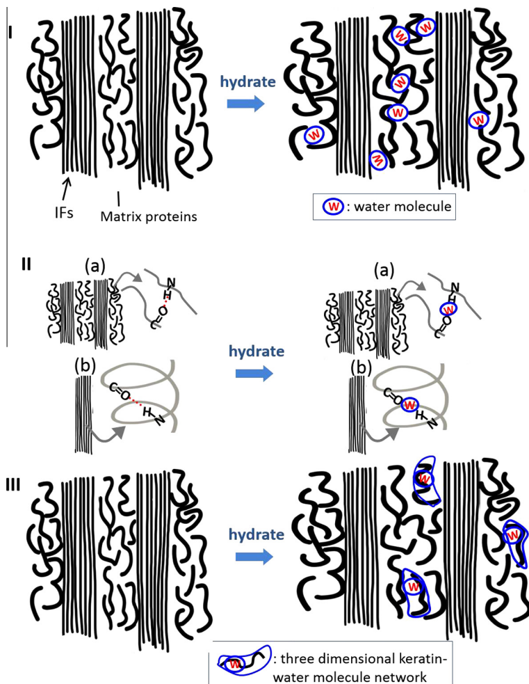
Fig. 15. Schematic diagrams of proposed water interaction with \alpha -keratin: (I) water act as cross links and a swelling agent to increase the distance between matrix proteins, (II) water may replace the hydrogen bonds in the matrix protein chains and/or in the IFs, and (III) in the matrix, water may form a three dimensional keratin–water network.
