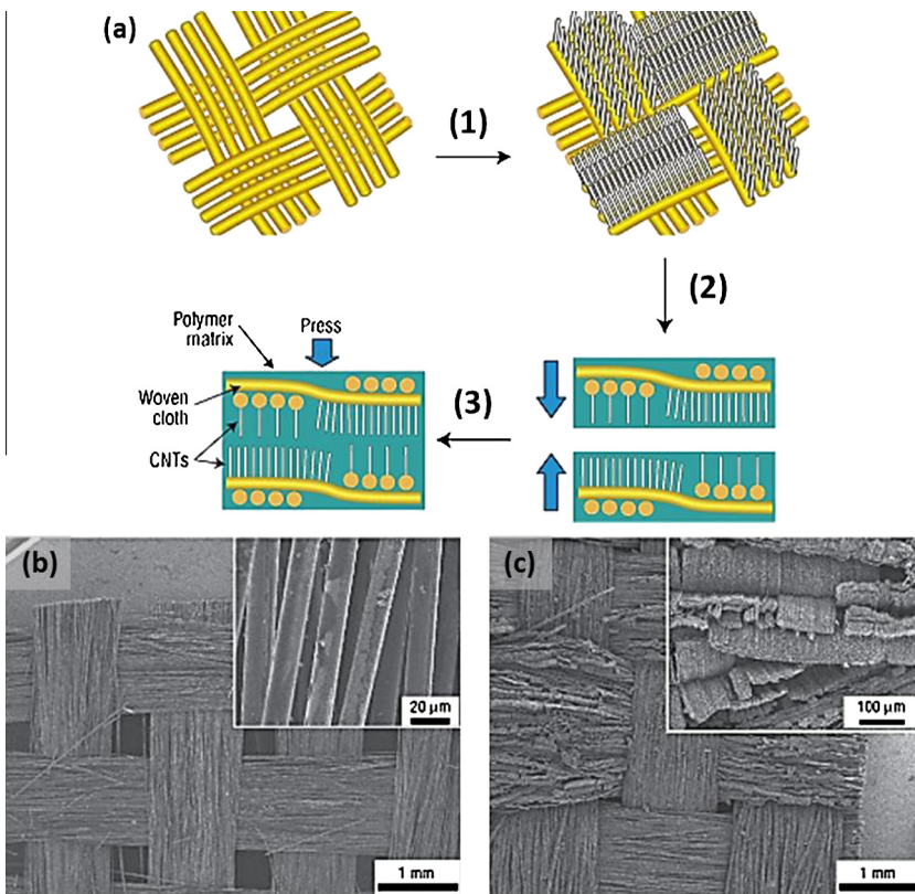
Fig. 76. (a) Processing for the manufacture of 3D carbon nanotubes (CNT) composite: (1) aligned CNTs grown perpendicular to SiC fiber cloth; (2) stacking of matrix-infiltrated (blue color) CNT-grown fiber cloth; (3) 3D nanocomposite plate fabrication by hand lay-up. (b) Scanning electron micrograph of the plain-weave SiC fabric cloth. Inset: higher magnification of the individual fibers. (c) Scanning electron micrograph of the cloth with CNTs grown perpendicularly on the surface. Inset: higher magnification image [308].
