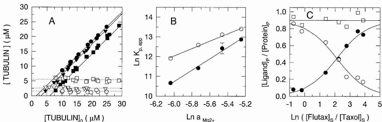
Fig. 3. A : Critical concentration ( C_r ) plots for GDP-tubulin assembly with taxol (circles, C_r 1.5 \mu\text{M} ), FLUTAX (triangles, C_r 2.6 \mu\text{M} ), and ROTAX (squares, C_r 5.5 \mu\text{M} ), under same conditions as Figure 2. The concentration of pelleted protein (filled symbols) and protein in the supernatant (open symbols) is plotted as a function of total tubulin concentration. B : Linkage graphs [Wyman and Gill, 1990] of the apparent elongation constant K_{p,app} = C_r^{-1} of FLUTAX (filled circles) and taxol-induced (open circles) polymerization of tubulin versus activity of \text{Mg}^{2+} ions. The slopes (2.9 and 1.9, respectively) are equal to the increment of \text{Mg}^{2+} ions preferentially bound by the tubulin polymer over the protomer. C : Competition of FLUTAX (filled circles) and taxol (open circles) for binding to microtubules assembled
