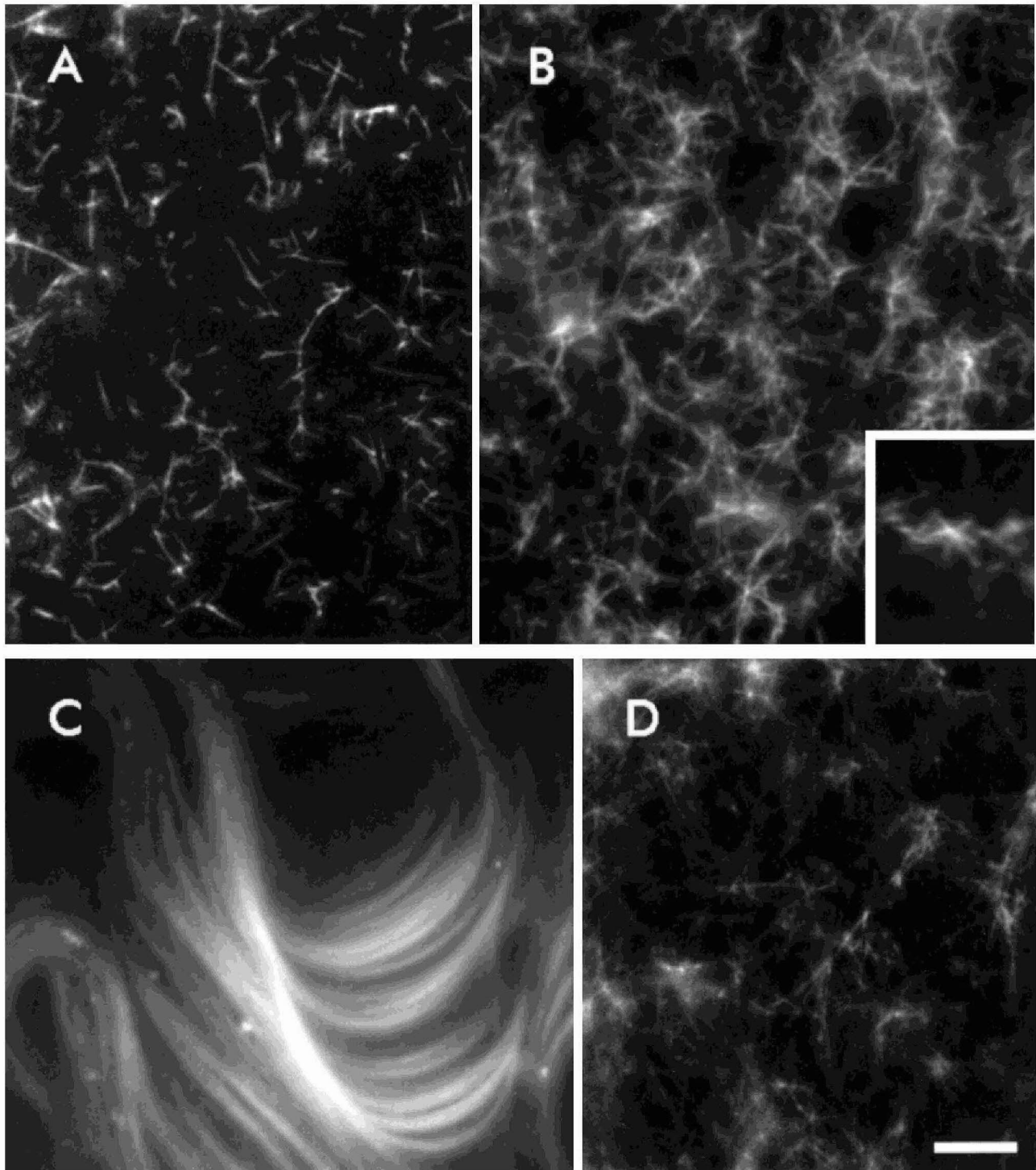
Fig. 5. Microtubules imaged with fluorescent taxoids under the epifluorescence microscope A : Microtubules assembled with 25 \mu\text{M} tubulin and FLUTAX. B : Another view of FLUTAX microtubules; inset : a radial aster-like formation of FLUTAX microtubules. C : Bundles of ROTAX microtubules. D : Microtubules assembled with MAPs and visualized immediately after addition of FLUTAX and dilution to 0.4 \text{mg ml}^{-1} microtubule protein. Bar = 10 \mu\text{m} .
