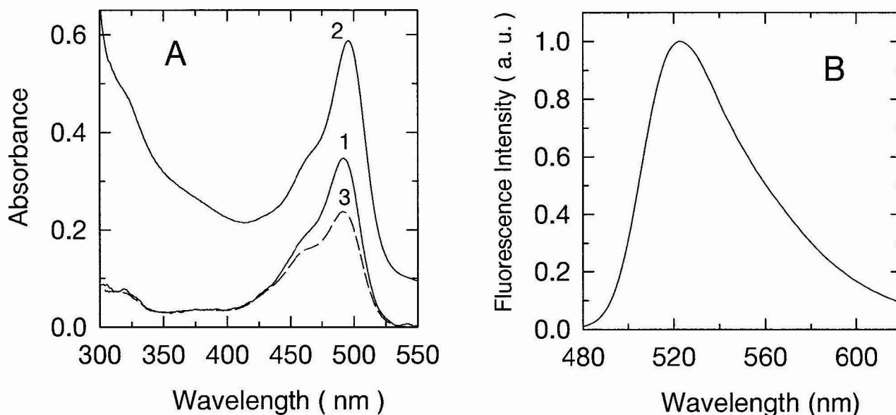
Fig. 4. A : Absorption spectra of free FLUTAX, 2 \mu\text{M} in PEGM buffer, pH 6.6 (line 1, absorbance multiplied by 10), FLUTAX bound to microtubules (20 \mu\text{M} , line 2; same conditions plus 25 \mu\text{M} tubulin, notice the light scattering due to microtubules) and free FLUTAX, 20 \mu\text{M} in the same buffer (dashed line 3, shown for comparison; notice the absorption changes due to FLUTAX aggregation). B : Corrected fluorescence spectrum of FLUTAX in microtubules ( \lambda_{ex} = 470 nm, slit 2 nm). The normalized spectrum of free FLUTAX in buffer was marginally wider at the red side.
