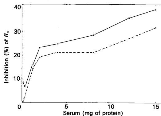
Fig. 3. Dose-responses of serum (□) and dialysed serum (Δ) on calcium phosphate precipitation
