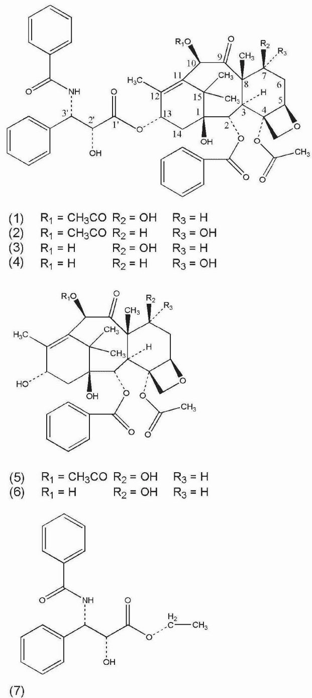
Figure 1. The structures of paclitaxel and related compounds: paclitaxel (1) 7-epi-taxol (2), 10-deacetyltaxol (3), 7-epi-10-deacetyltaxol (4), baccatin III (5), 10-deacetylbaccatin III (6) and N -benzoyl-3-phenylisoserine ethyl ester (7).
