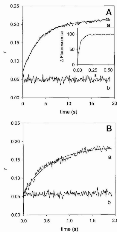
FIG. 6. A, kinetics of binding of Flutax-1 to microtubules at 37 °C. In the anisotropy stopped-flow device, a 1 μM solution of Flutax-1 was mixed with 24 μM pure tubulin assembled into microtubules (concentration of sites 20 μM) (final concentrations of 500 nM Flutax and 10 μM) in the absence (a) and presence (b) of 50 μM docetaxel. Inset, kinetics of binding of Flutax-1 of the same sample followed by the change in fluorescence intensity. B, kinetics of binding of Flutax-2 to microtubules at 37 °C. In the anisotropy stopped-flow device, a 1 μM solution of Flutax-2 was mixed with 24 μM pure tubulin assembled into microtubules (concentration of sites 20 μM) (final concentrations of 500 nM Flutax and 10 μM sites) in the absence (a) and presence (b) of 50 μM docetaxel. Curve a is fitted to an exponential decay.
