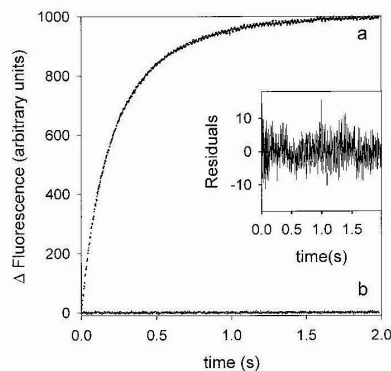
FIG. 5. Kinetics of binding of 5 μM Flutax-1 to 5 μM sites in microtubules assembled from pure tubulin in GAB in the absence (a) and presence (b) of 100 μM docetaxel. The data were fitted using the reaction model 1; the obtained kinetic constants were k_{+1} = 6.30 \pm 0.10 \times 10^6 \text{ M}^{-1} \text{ s}^{-1} and k_{-1} = 1.17 \pm 0.38 \times 10^{-2} \text{ s}^{-1} (see Table III for comparison). Inset, residues between the experimental and theoretical curves.
