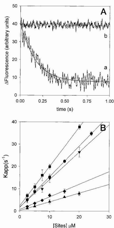
FIG. 4. A, kinetics of binding of Flutax-2 to microtubules at 35 °C. A 500 nM solution of Flutax-2 was mixed with 20 μM sites in cross-linked microtubules of pure tubulin in GAB in the stopped-flow device (final concentrations of 250 nM Flutax-2 and 10 μM sites) in the absence (a) and presence (b) of 50 μM docetaxel. The solid line is the best fit. Data were averaged in 5-ms intervals. B, dependence on the concentration of sites in the cross-linked microtubules of the observed rate constants of binding of Flutax-2 (250 nM) at 32 °C (triangles), 35 °C (diamonds), 37 °C (circles), 39 °C (inverted triangles), and 42 °C (squares) to microtubules assembled from pure tubulin in GAB. The solid lines are the best fittings to the experimental data.
