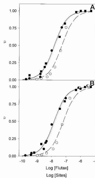
FIG. 2. A, solid line and circles, titration curve of 1 \mu\text{M} taxoid sites in stabilized microtubules with Flutax-1 at 27 ^{\circ}\text{C} measured by centrifugation; data are corrected for the percentage of inactive ligand. Dashed line and open circles, uncorrected data and fit. A small part of the ligand in use was found to be inactive, since it remained in the supernatant at very high concentrations of microtubules, disturbing the measurement of the free ligand concentration and artifactually decreasing the apparent binding constant measured. This effect was corrected as described under "Experimental Procedures." This percentage was found to be 4 \pm 1\% in the case of Flutax-1 and 6 \pm 1\% in the case of Flutax-2. Solid squares and dotted line, titration curve of 25 nM Flutax-1 with taxoid sites in stabilized microtubules measured by anisotropy. B, solid line and circles, titration curve of 1 \mu\text{M} taxoid sites in stabilized microtubules with Flutax-2 at 27 ^{\circ}\text{C} corrected for the percentage of inactive ligand. Dashed line and open circles, uncorrected data. Solid squares and dotted line, titration curve of 25 nM Flutax-2 with stabilized microtubules measured by anisotropy.
