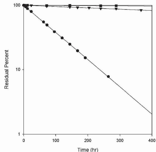
Figure 2. Semi-log plots for the degradation of 10-deacetylbaccatin III in aqueous solution at pH 1.09 (●), pH 1.99 (▼), and pH 3.05 (■), T = 25^\circ\text{C} showing the loss of 10-deacetylbaccatin III follows pseudo-first-order kinetics.
