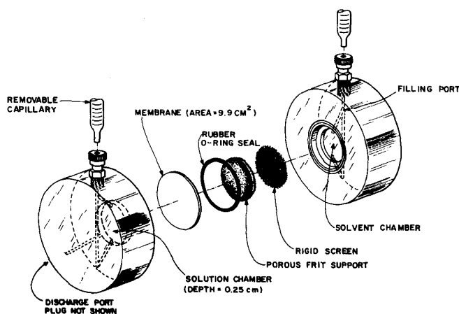
FIG. 2. Exploded view of the membrane osmometer cell.
