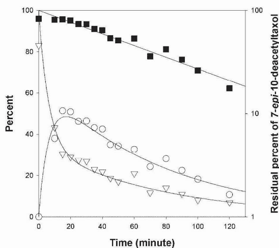
Figure 11. Time courses for the loss of S -epimer (▽), formation and loss of R -epimer (○), and total 7- epi -10-deacetyltaxol disappearance (■, total of the S - and R -epimers) at pH 7.72 and 70°C. The total 7- epi -10-deacetyltaxol is plotted semilogarithmically versus time. The solid lines represent the best fit to Eqs. (9)–(11).
