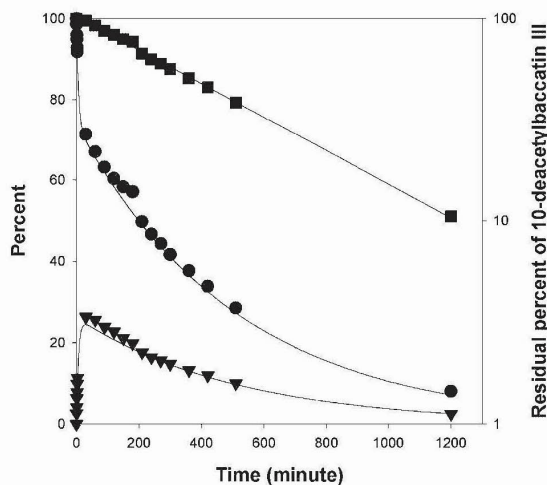
Figure 3. Time courses for the loss of S -epimer (●), formation and loss of R -epimer (▼), and total 10-deacetylbaecatin III disappearance (■, total residual of the S - and R -epimers) at pH 10.8 and 25°C. The total residual of 10-deacetylbaecatin III is plotted semilogarithmically versus time. The solid lines represent the best fit to Eqs. (9)–(11).
