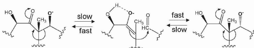
Scheme 3. Proposed mechanism for epimerization of 10-deacetylbaccatin III.
