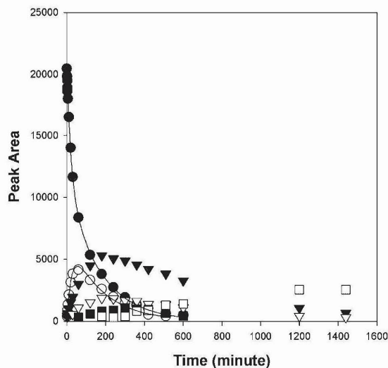
Figure 5. Time course of the degradation of baccatin III in aqueous solution at pH 10.77, T = 25^\circ\text{C} . Symbol key: baccatin III (●); baccatin V (7- epi -baccatin III, ○); 10-deacetylbaccatin III (▼); 7- epi -10-deacetylbaccatin III (▽); unidentified product 1 (■); unidentified product 2 (□). The solid lines represent the best fit to the Eqs. (9) and (10), according to the measured loss of baccatin III (●), formation and loss of baccatin V (7- epi -baccatin III, ○).
