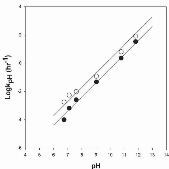
Figure 6. pH-rate profile for the values k_1 (●) and k_2 (○) used to describe the epimerization of 10-deacetylbaccatin III at various pH values, 25°C. The solid line represents the best fit to Eq. (12) where k_{1B} = 4.92 \pm 0.82 \times 10^3 \text{ M}^{-1} \text{ h}^{-1} ; k_{2B} = 1.24 \pm 0.13 \times 10^4 \text{ M}^{-1} \text{ h}^{-1} .
