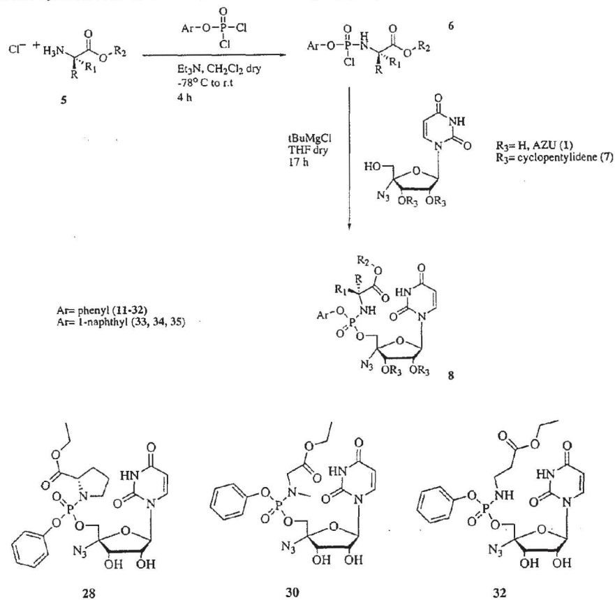
Scheme 2. General Synthetic Pathway for the Deprotection of 2'-3'-cyclopentylidene AZU Phenyl-phosphoramidates
