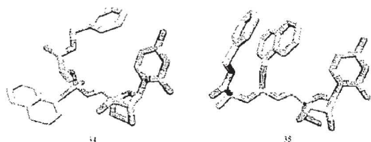
Figure 2. Lowest energy conformations of compounds 34 and 35.
