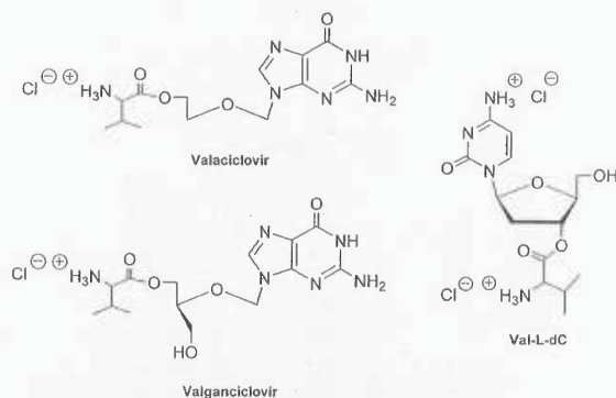
Figure 2. Structures of valaciclovir, valganciclovir, and val-L-dC.
