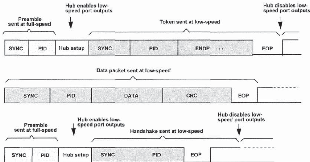
Figure 8-48. Low-speed Transaction
