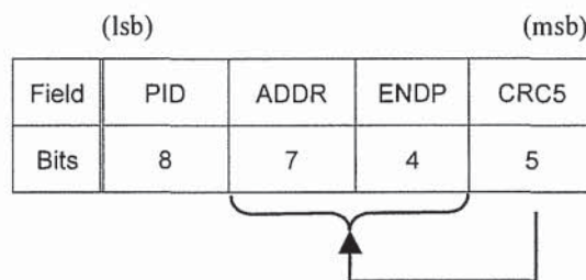
Figure 8-5. Token Format
