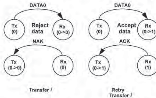
Figure 8-17. NAKed Transaction with Retry
