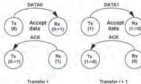
Figure 8-16. Consecutive Transactions
