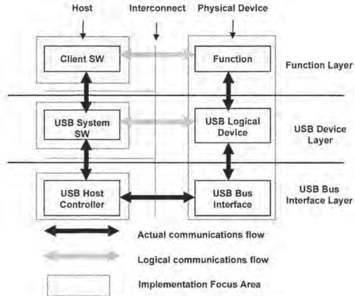
Figure 5-2. USB Implementation Areas
