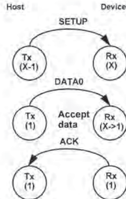
Figure 8-15. SETUP Initialization
