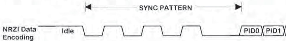
Figure 7-25. Sync Pattern
