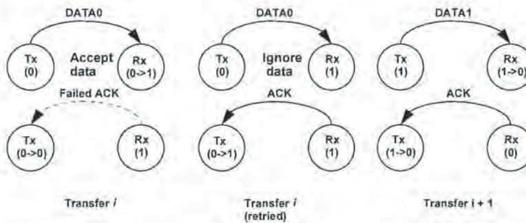
Figure 8-18. Corrupted ACK Handshake with Retry
