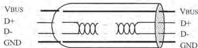
Figure 4-2. USB Cable
