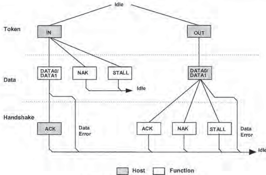
Figure 8-9. Bulk Transaction Format
