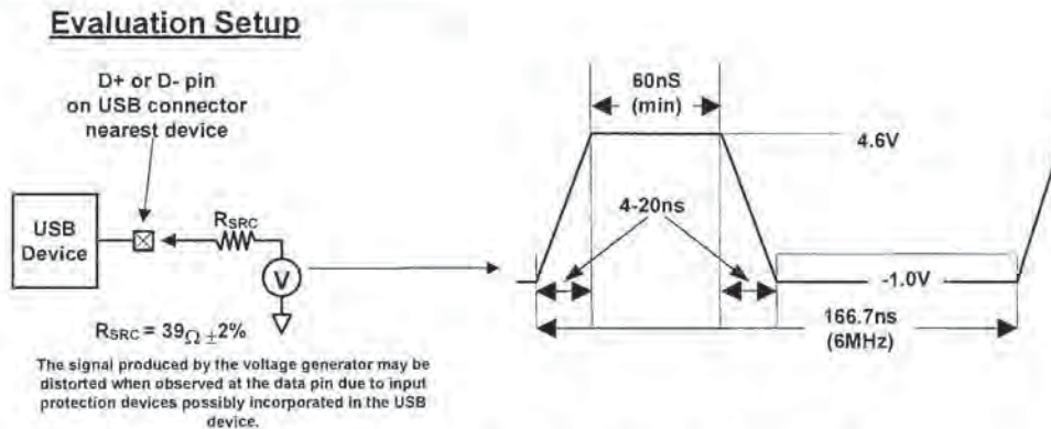
Figure 7-1. Maximum Input Waveforms for USB Signaling
