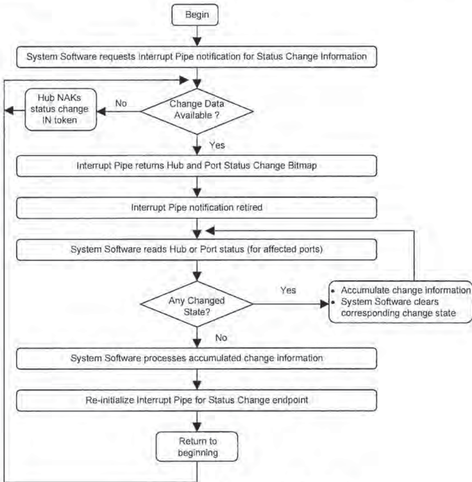
Figure 11-13. Port Status Handling Method
