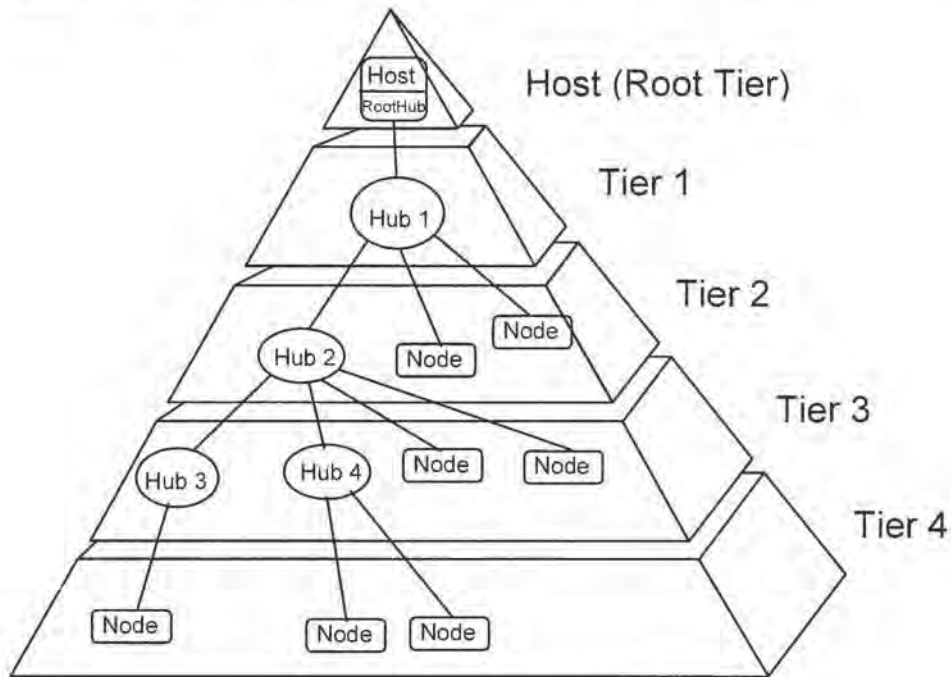
Figure 4-1. Bus Topology
