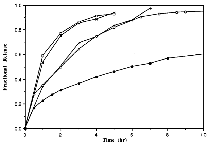
Fig. 2. In vitro release profiles of different types of hydrophilic matrices of ABT-089 containing [x] 26% Methocel K100M (H1); [□] 25% Polyox coagulant (H2); [+] 35% Methocel K100M with hydrophilic barrier layers (HHH) and [○] 35% Methocel K100M with hydrophobic barrier layers (WHW) compared with a hydrophobic matrix containing [●] 55% Carnauba wax (W2) (24 h data not shown).
