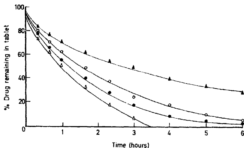
Fig. 1. The release of chlorpheniramine from different viscosity grade HPMCs. Key: Methocel E5, \Delta ; Methocel E15, \bullet ; Methocel E50, \bullet ; Methocel E4M, \Delta .
