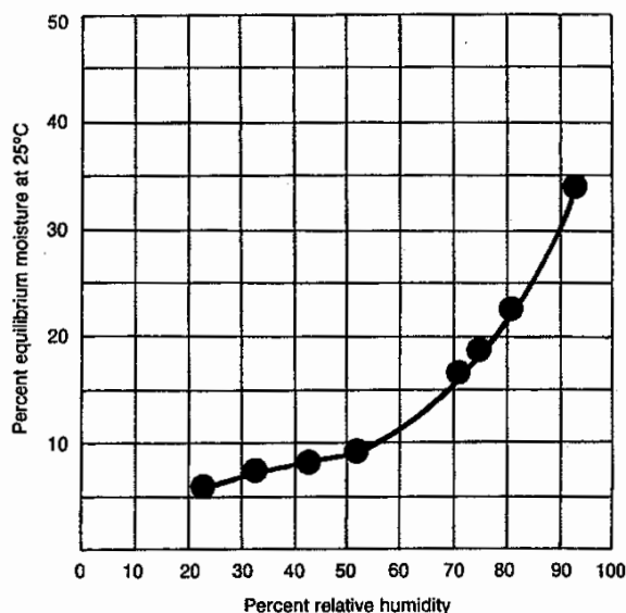
Fig. 1: Moisture sorption isotherm of methylcellulose.
