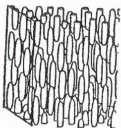
Figure 3-9 Nematic phase
