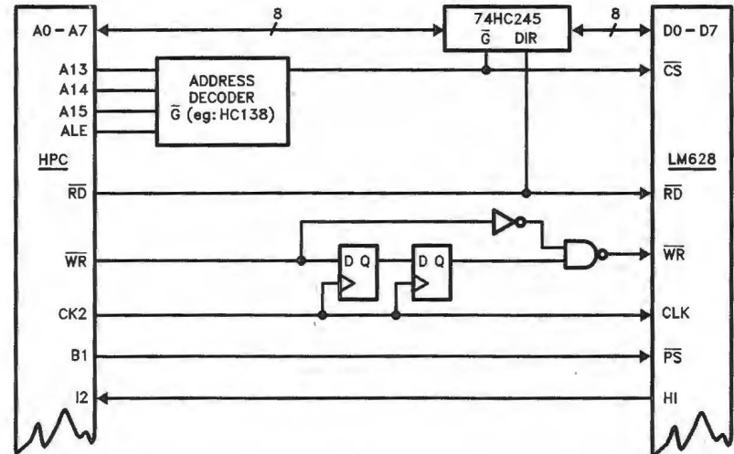
FIGURE 13. LM628 and HPC Interface
