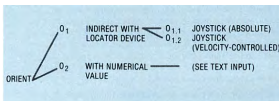
Figure 3. Orienting techniques.
