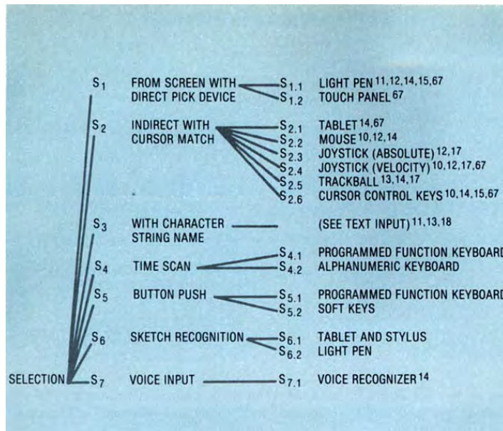
Figure 1. Selection techniques.
