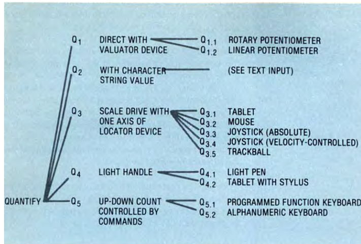
Figure 4. Quantifying techniques.
