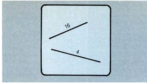
Figure 14. Labeled lines.
