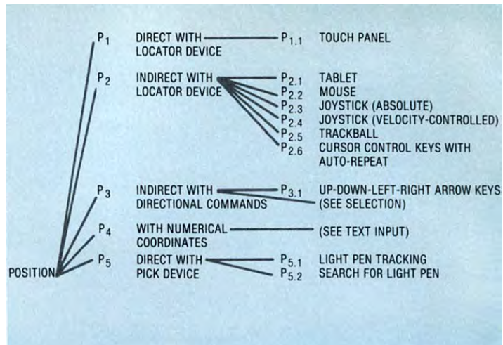
Figure 2. Positioning techniques.
