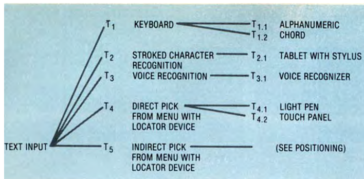
Figure 5. Text-entry techniques.
