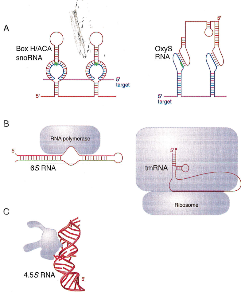
Fig. 1. Different mechanisms of ncRNA (red) action. (A) Direct base-pairing with target RNA or DNA molecules is central to the function of some ncRNAs: Eukaryotic snoRNAs direct nucleotide modifications (green star) by forming base pairs with flanking sequences, and the E. coli OxyS RNA represses translation by forming base pairs with the Shine-Dalgarno sequence (green box) and occluding ribosome binding. (B) Some ncRNAs mimic the structure of other nucleic acids: Bacterial RNA polymerase may recognize the 6S RNA as an open promoter, and bacterial ribosomes recognize tmRNA as both a tRNA and an mRNA. (C) ncRNAs also can function as an integral part of a larger RNA-protein complex, such as the signal recognition particle, whose structure has been partially determined (49).
