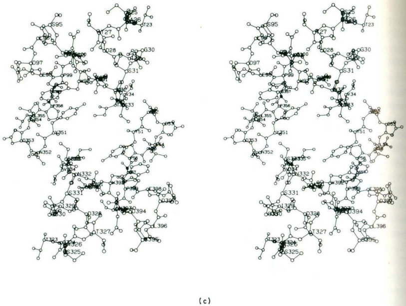
FIG. 13. Contacts across the 2-fold axis of dimerization. (a) Upper region near the top of the cavity; (b) lower region at the base of the cavity; (c) all hypervariable residues.
