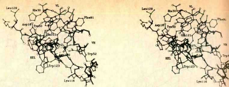
Fig. 4. Stereo diagram of the antibody-antigen interface in a similar orientation to Fig. 1. All atoms are shown for those residues involved in the interaction. Heavy and light main chains are indicated by thick and thin bonds, respectively, and hydrogen bonds by dotted lines. Lysozyme residues broadly lie below the diagonal from top left to lower right of the diagram.
