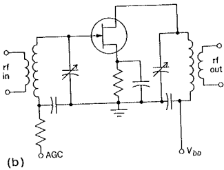
Typical radio-frequency amplifier circuits with (a) bipolar transistor and (b) field-effect transistor. AGC = automatic gain control; VCC = collector supply voltage; VDD = drain supply voltage.
