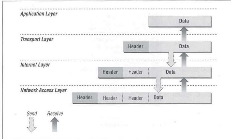
Figure 1-3: Data encapsulation
