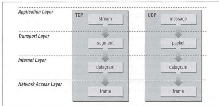
Figure 1-4: Data structures
