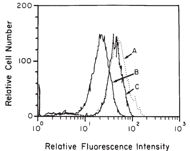
Fig. 2. Inhibition of binding of FITC-anti-Leu-3a to A3.01 cells by anti-Id mAb HF1.7. The A3.01 cells were stained with FITC-anti-Leu-3a in the presence of PBS (trace A) or PBS containing 10 \mu g of HF1.7 (trace B) or 10 \mu g of GB-2 (trace C).
