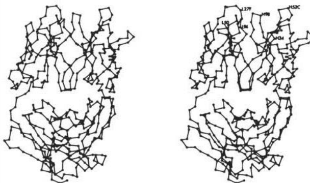
FIG. 4. Stereo view of the C_\alpha skeleton of the J539 Fab structure. Open circles, McPC603 hypervariable residues that were excluded from the search.
