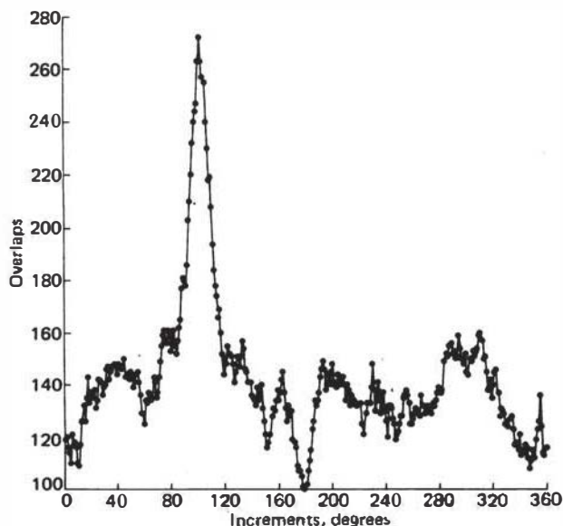
FIG. 2. Overlap of domain pair C H1 -C L on the J539 4.5-Å electron-density map as a function of the single Eulerian angle θ 1 . The angle was systematically varied in 1° intervals over its full range with all other rotation and translation variables fixed at their maximal overlap values.
