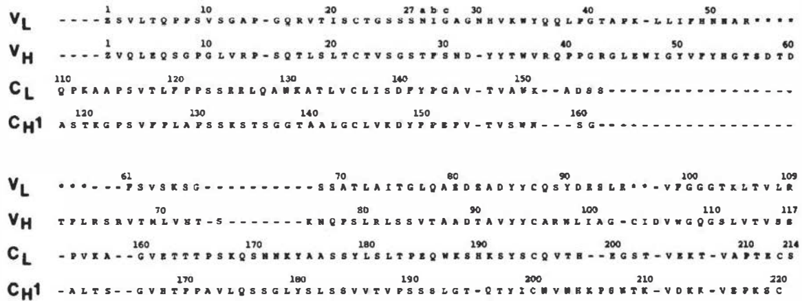
FIG. 4. Amino acid sequences of the V_L , C_L , V_H , and C_H1 homology regions of Fab New aligned by comparison of their three-dimensional structures. --- indicate gaps introduced to maximize alignment of the three-dimensional structures. * indicate deletions in the V_L sequence. See Ref. 11 for the V_L and C_L sequences, Ref. 12 for V_H , and Ref. 13 for C_H1 . Abbreviations for amino acids are as given in Ref. 14.
