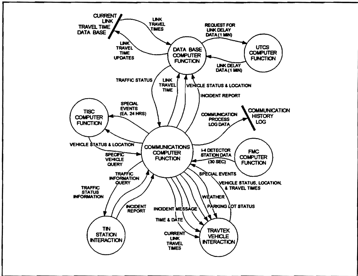
Figure 23. TMC communications data flow.
