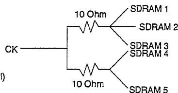
Figure 4.5.4-H 168 Pin UNBUFFERED DRAM DIMM CLOCK WIRING
