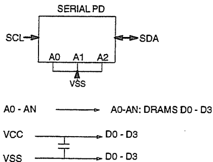
Figure 4.5.5-1 144 Pin X64 DRAM SO-DIMM, 1 Bank with X16 DRAMs
