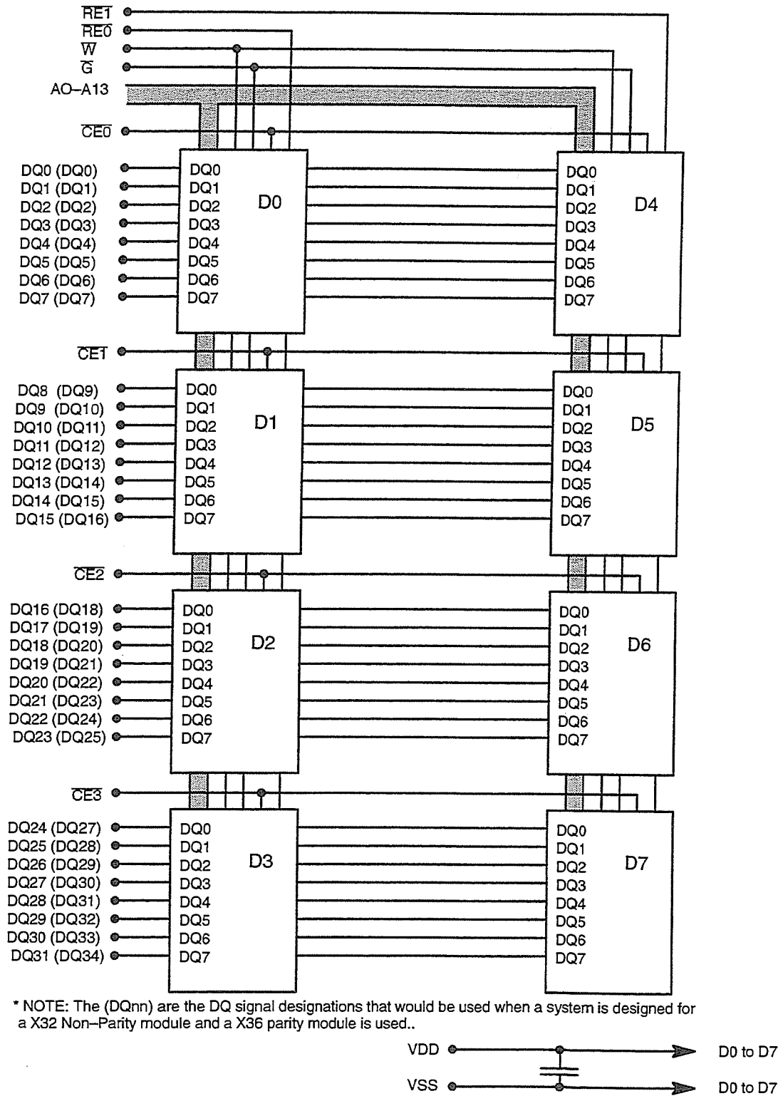
FIGURE 4.4.5-D X 32 DRAM SO-DIMM USING X8 DEVICES
