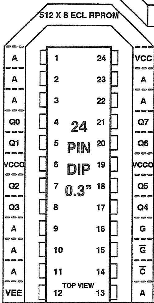
FIGURE 3.3.2-11 512 BY 8 10K & 100K ECL RPPROM
