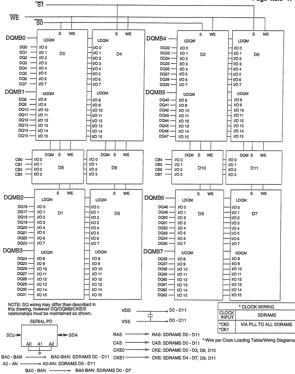
Figure 4.5.6-P 144 Pin X72 ECC SDRAM SO-DIMM, 2 Bank with X16 & X4 DRAMs
