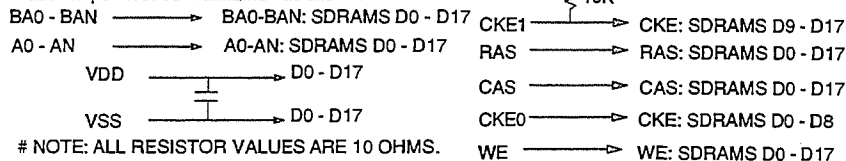
Figure 4.5.4-S X72 ECC SDRAM DIMM, 2 Banks with X8 SDRAMs
