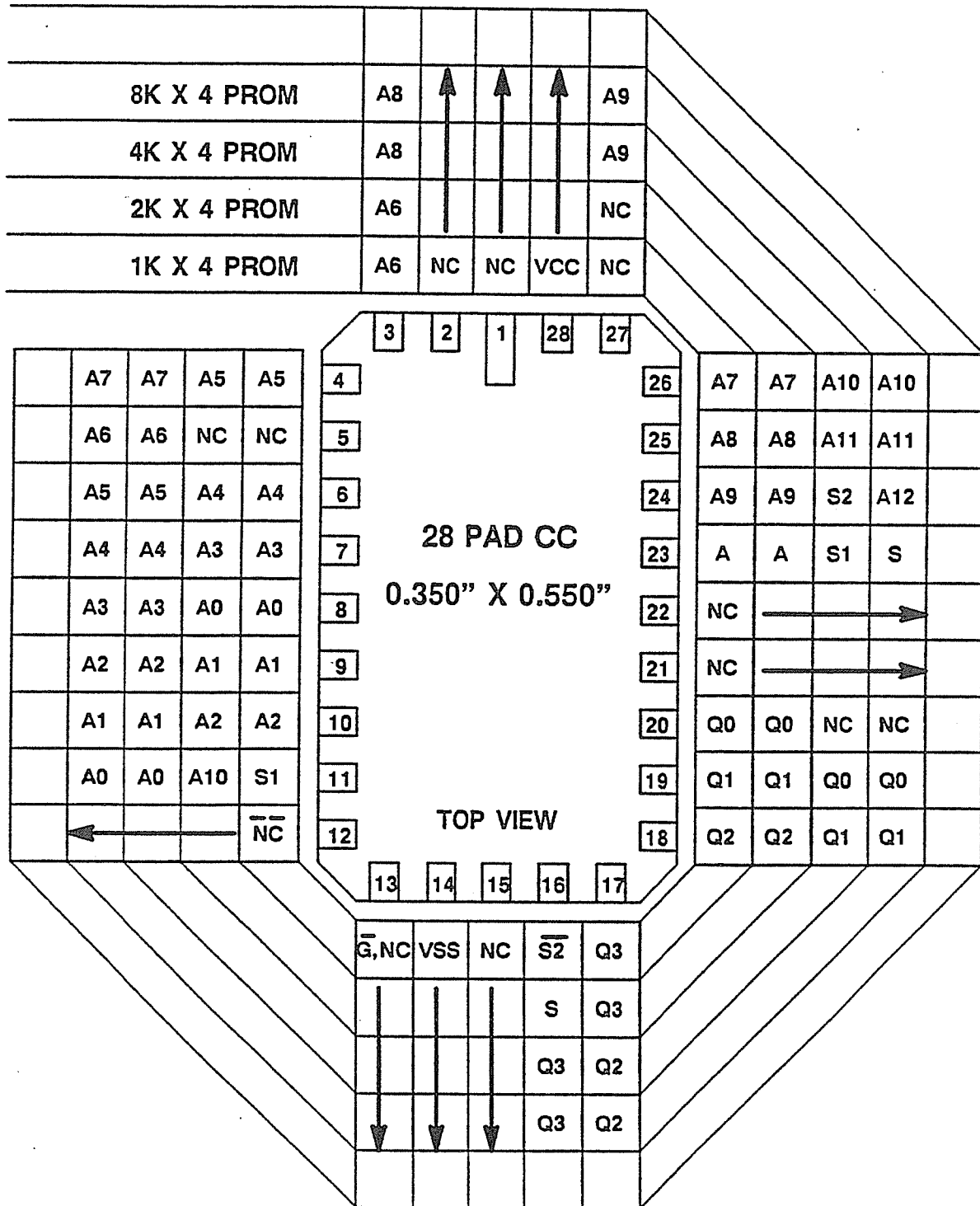
FIGURE 3.3.1-6 1K TO 8K BY 4 TTL PROM IN RCC
