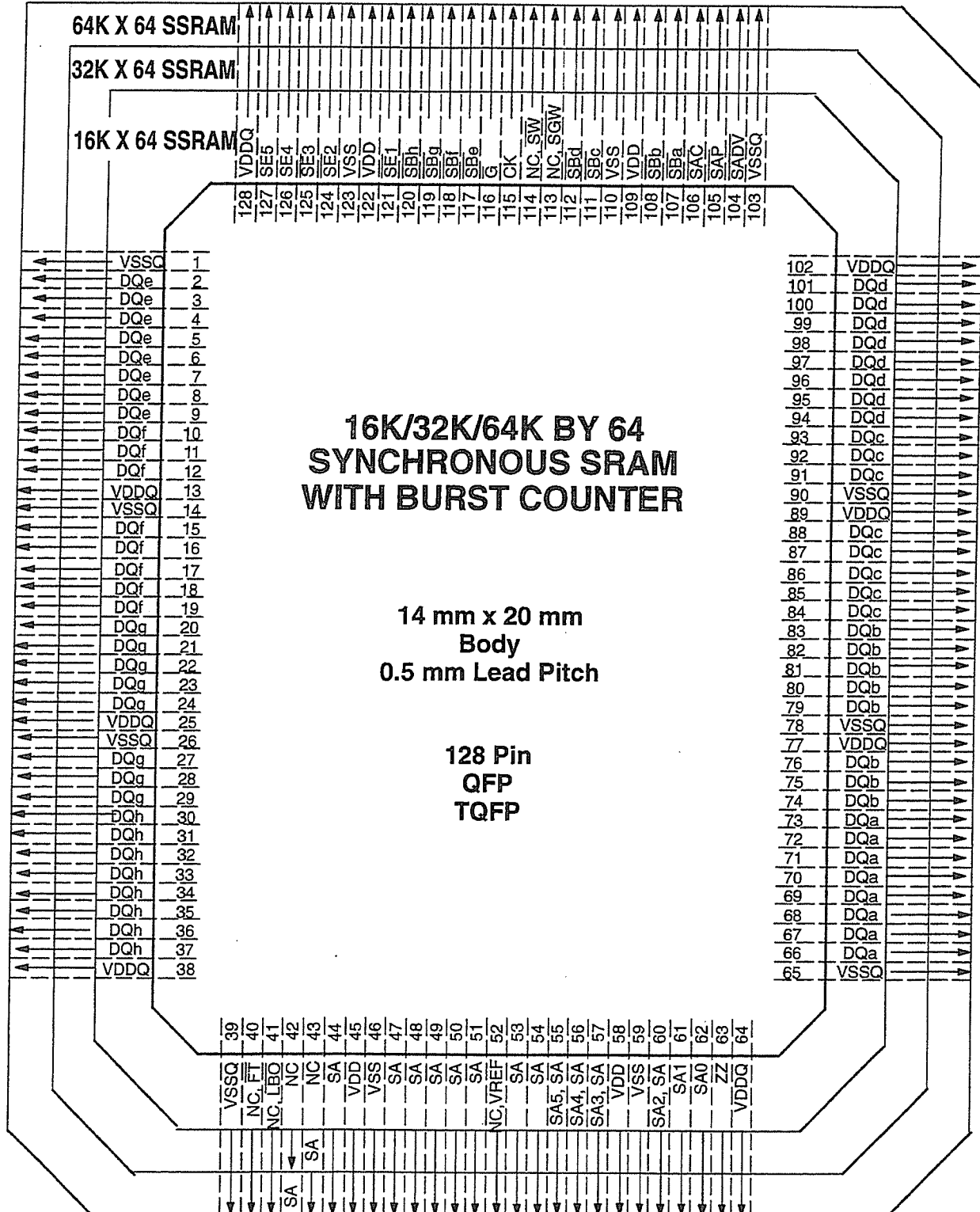
FIGURE 3.7.8-6 16K/32K/64K BY 64 SYNCHRONOUS SRAM WITH BURST COUNTER
