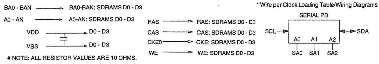
Figure 4.5.4-K X64 SDRAM DIMM, 1 Bank with X16 SDRAMs
