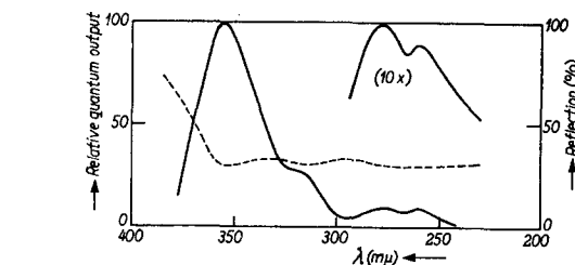
FIG. 3. Diffuse reflection spectrum (broken line) and relative excitation spectrum (solid line) of the Ce 3+ fluorescence of Sc 0.99 Ce 0.01 BO 3 .
